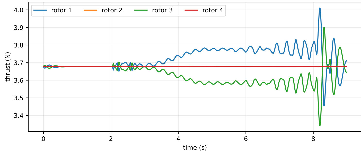
Rotor thrusts during contact
