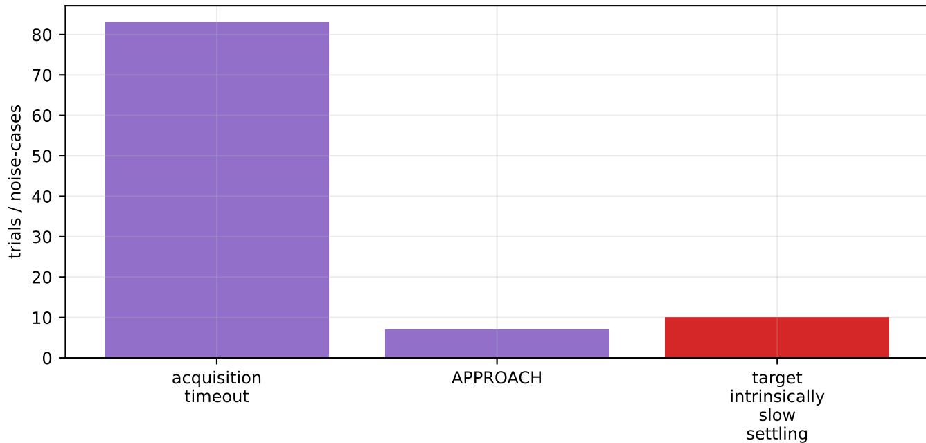
Failure mechanisms: delivery failures and false-safe audit
