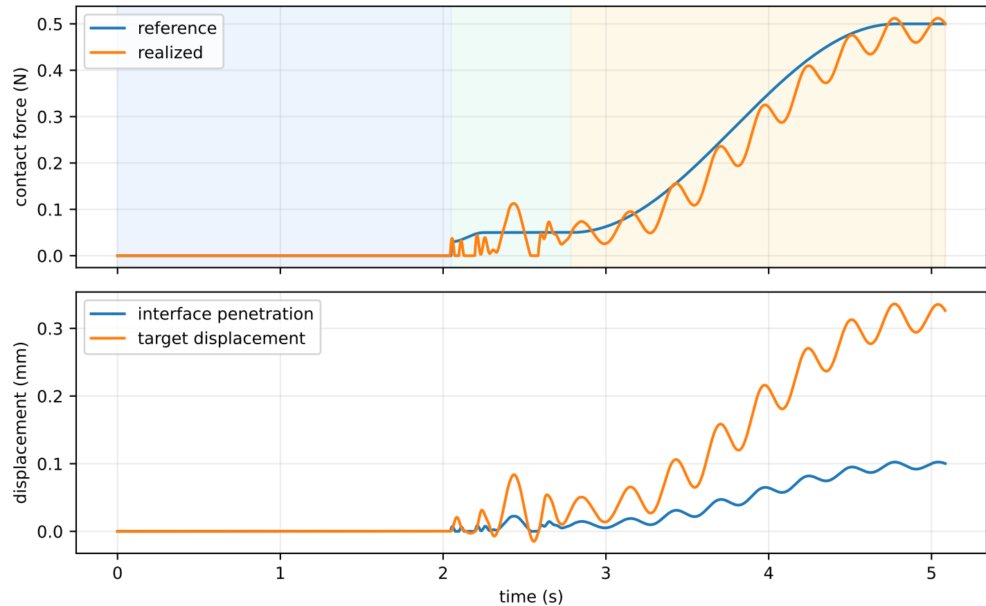
Slow approach and stable contact acquisition
