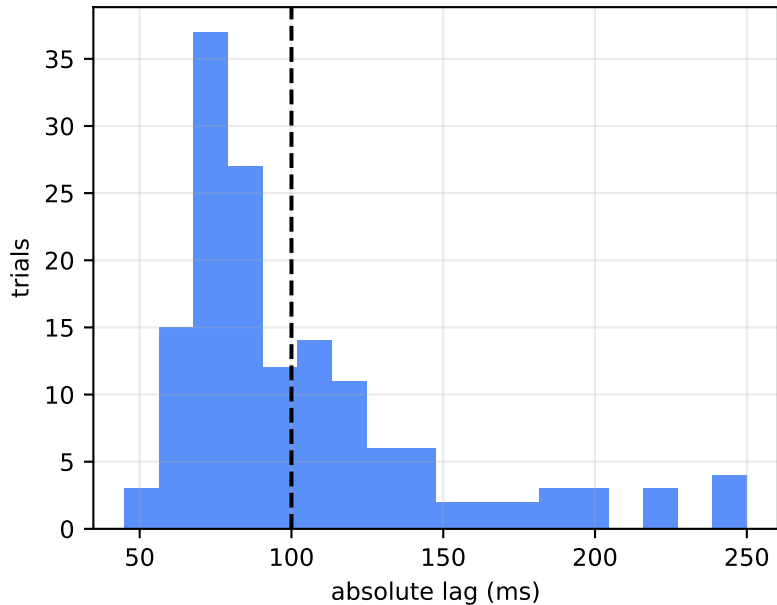
Completed-trial phase lag
