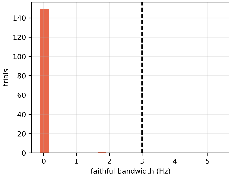
99.3% have no faithful bin
