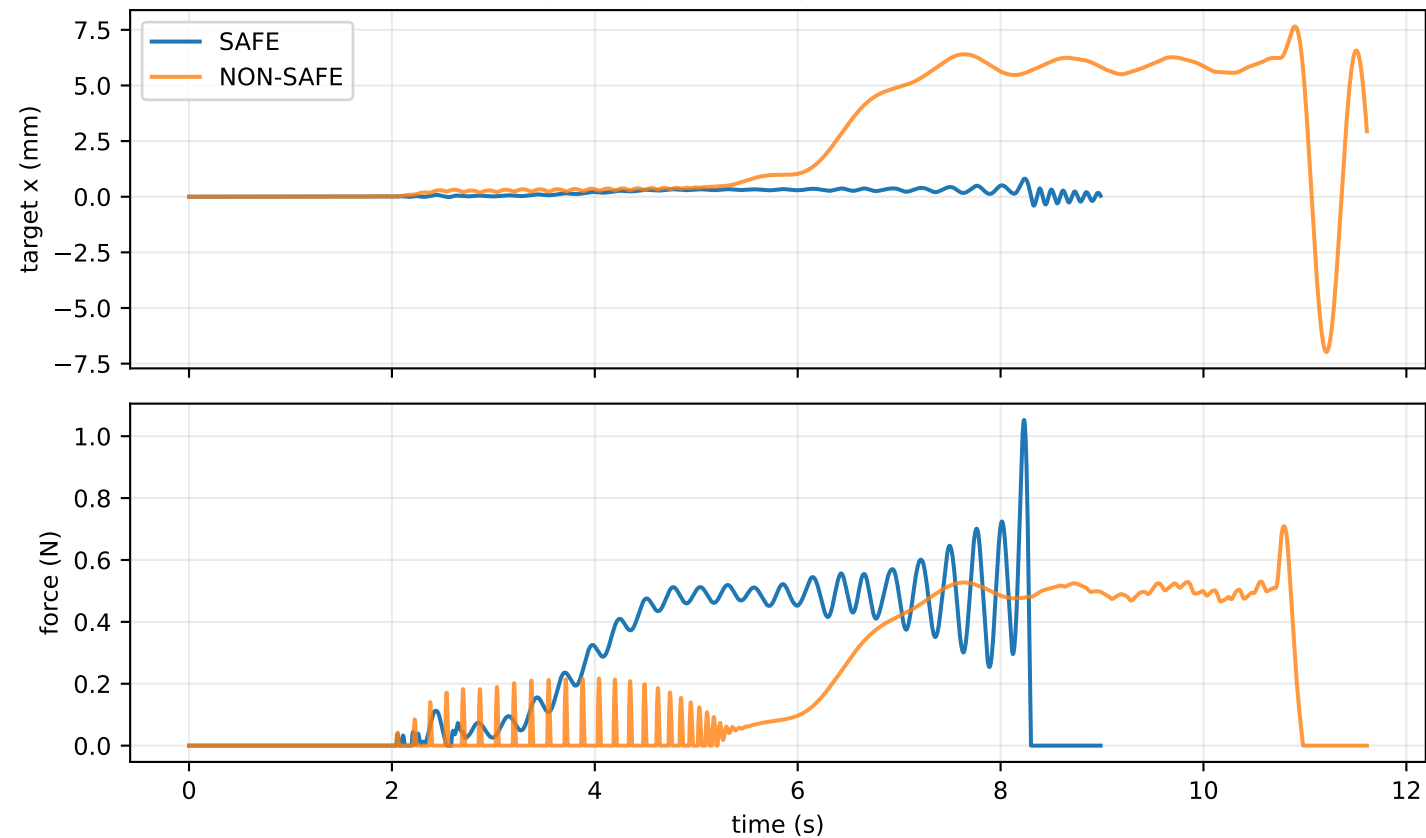
Target response and passive ring-down
