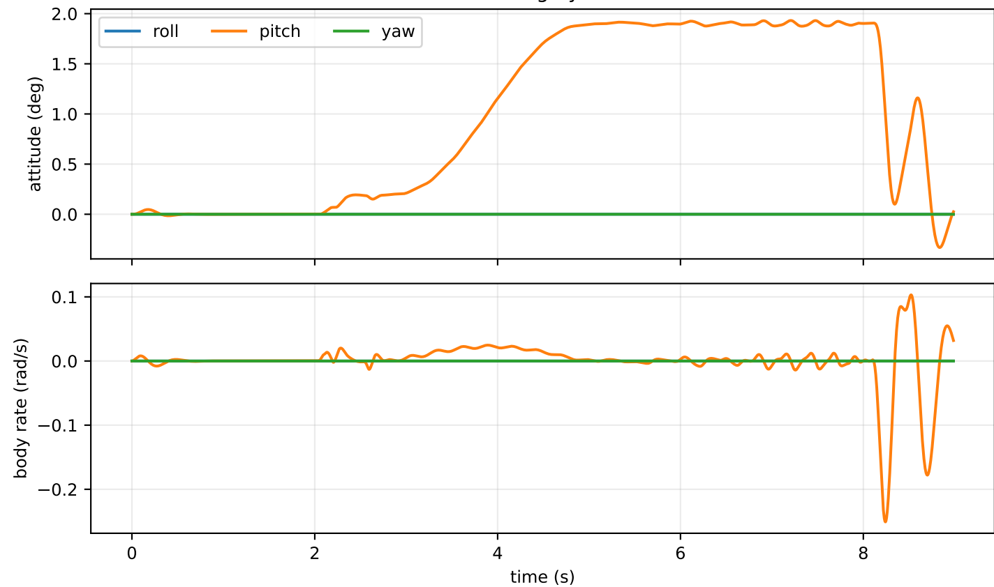
UAV attitude during hybrid interaction
