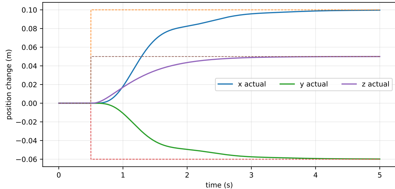
3-D translational controller validation
