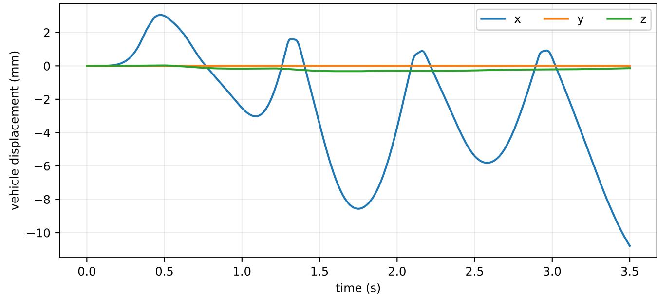
UAV motion during probing
