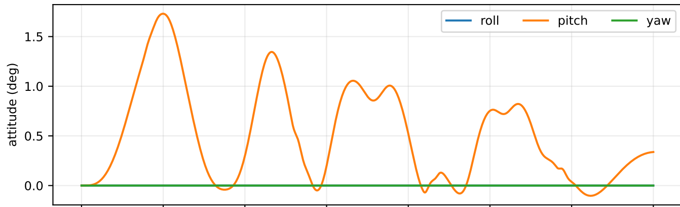
Offset-contact attitude disturbance
