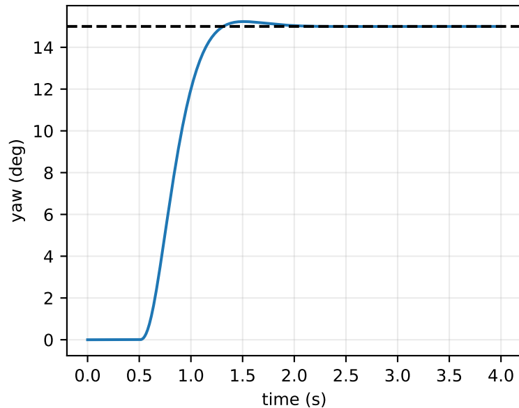
15° yaw step
