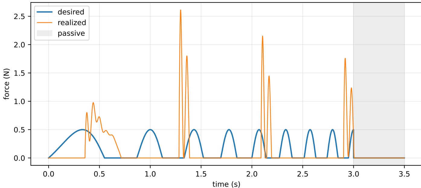
Desired versus realized probe — stiff target
