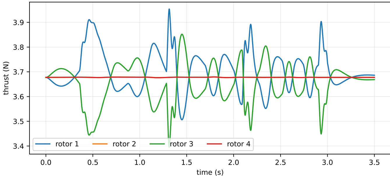
Individual rotor thrusts during contact
