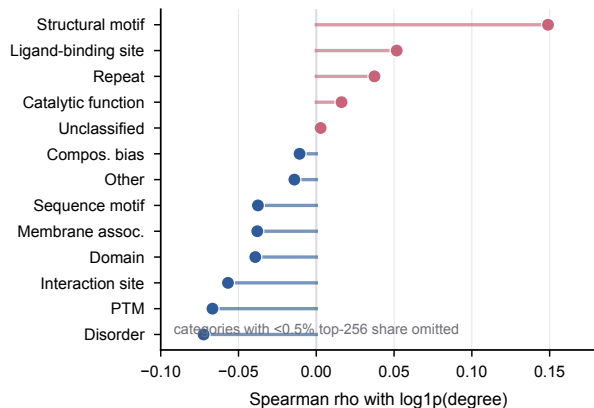
c Most SAE category shifts are weak but consistent
