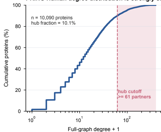
a PRING Human degree distribution is strongly skewed
