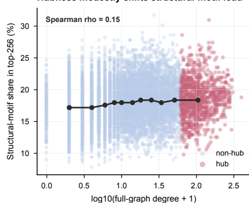
b Hubness modestly shifts structural-motif load
