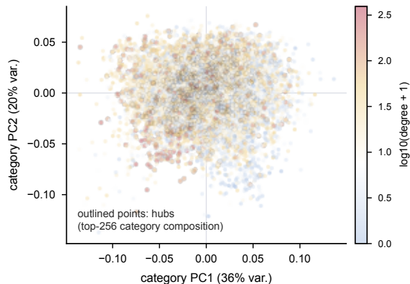
d Hub proteins occupy a shifted SAE category landscape
