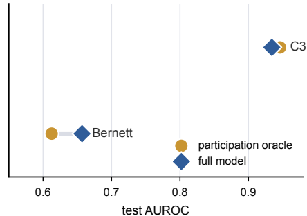
b Oracle tracks the model
