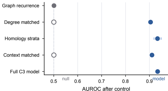
c Candidate leakage controls
