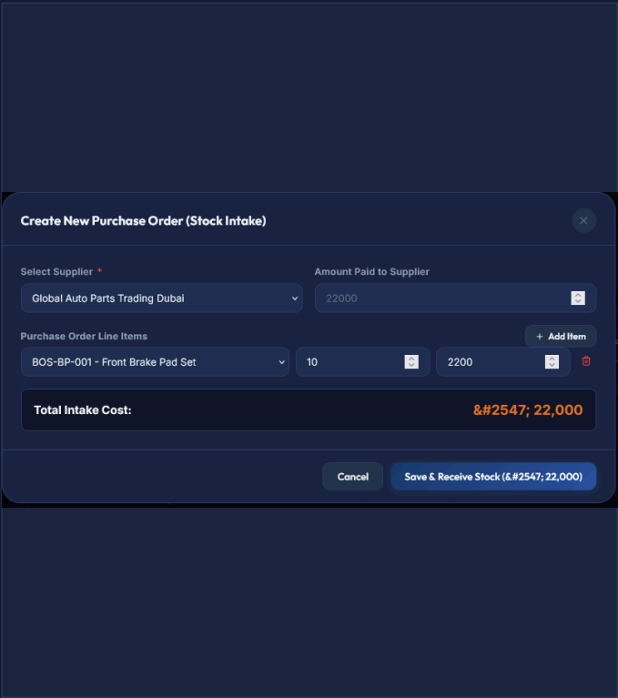
Create New Purchase Order · supplier & items
