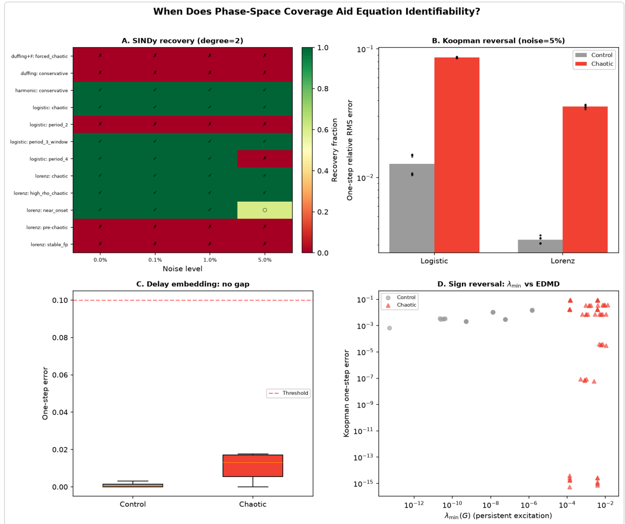
Figure 1: (A) SINDy recovery grid across all regimes and noise levels. (B) Koopman/EDMD reversal at noise=5%. (C) Delay-embedding closes the gap. (D) \lambda_{\min}(G) sign reversal for EDMD vs. SINDy's own predictor.
