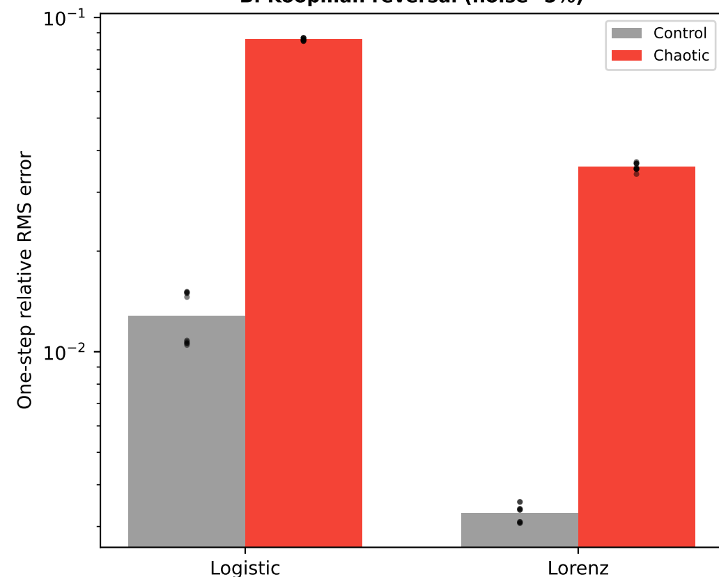
B. Koopman reversal (noise=5%)
