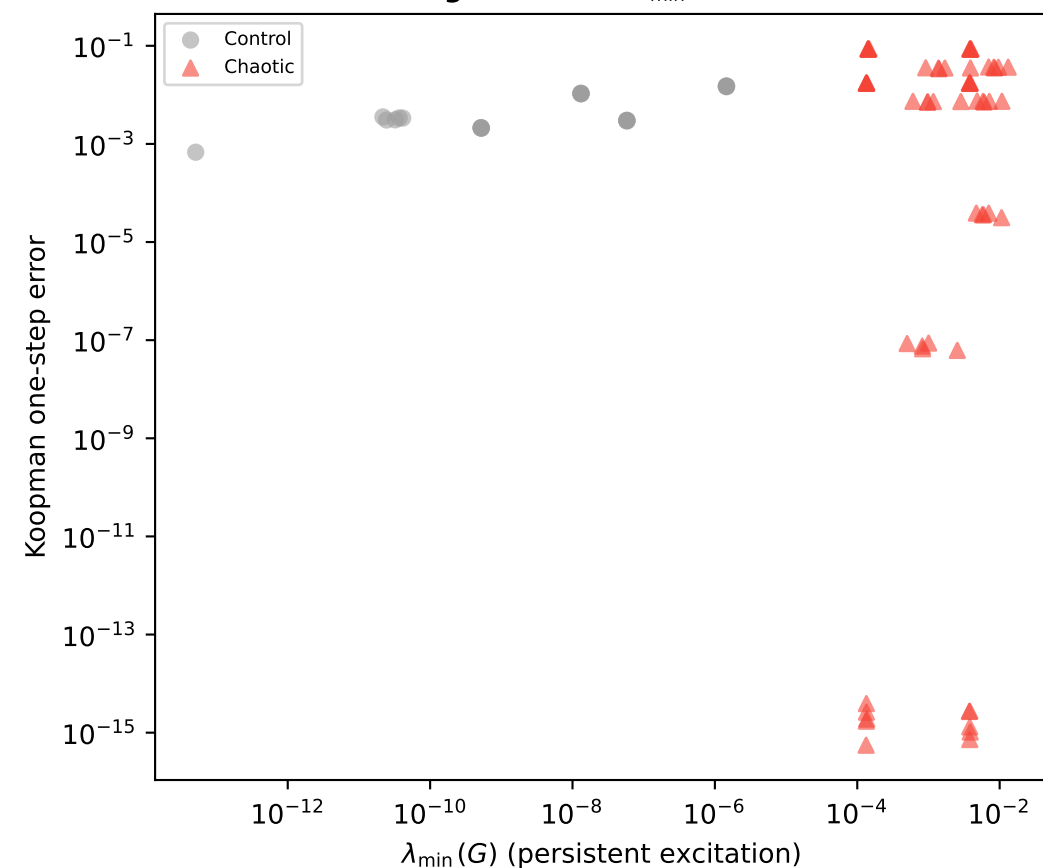
D. Sign reversal: \lambda_{\min} vs EDMD
