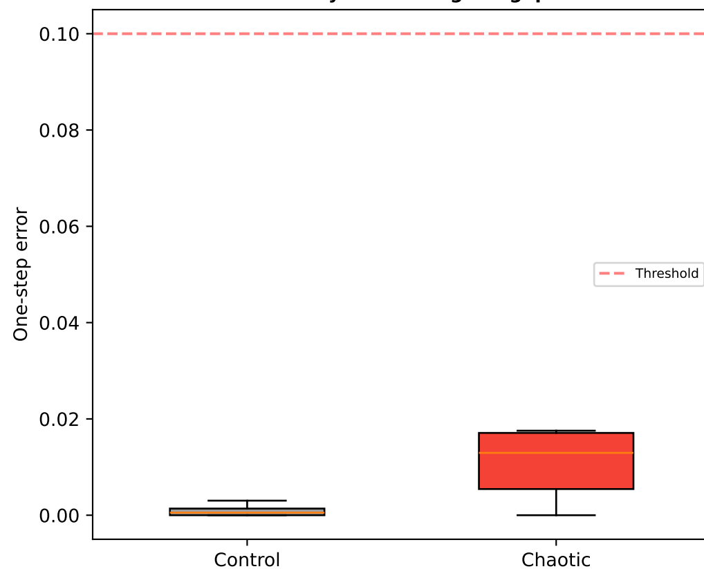
C. Delay embedding: no gap
