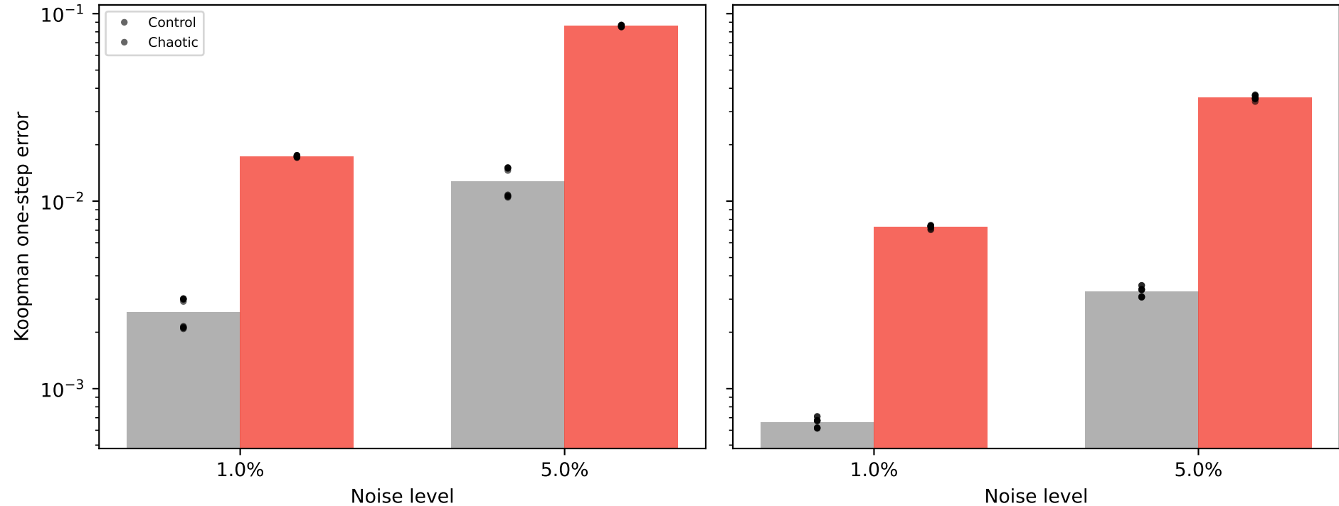
Logistic map
