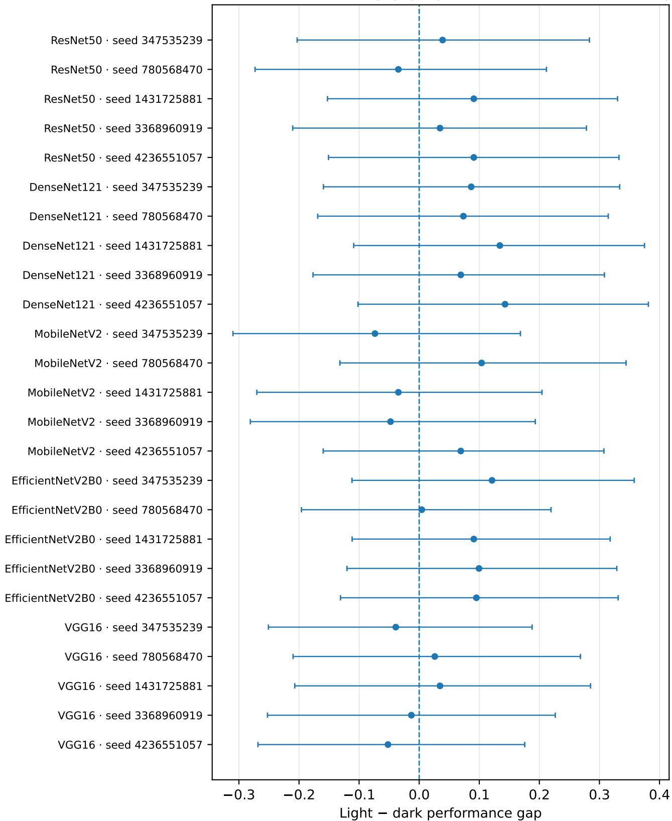
BOSQUE Recall / sensitivity gap by locked architecture-seed system
