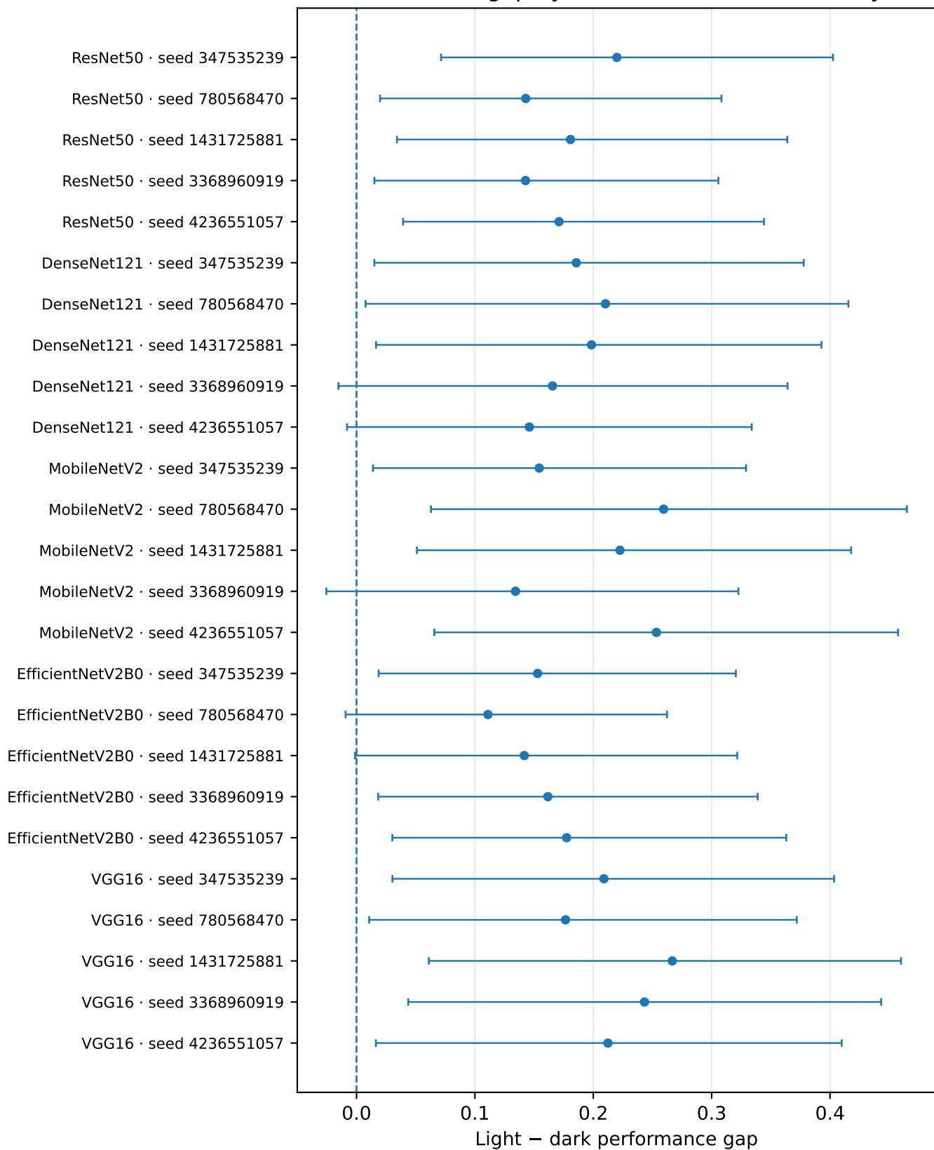
BOSQUE AUC-PR gap by locked architecture-seed system
