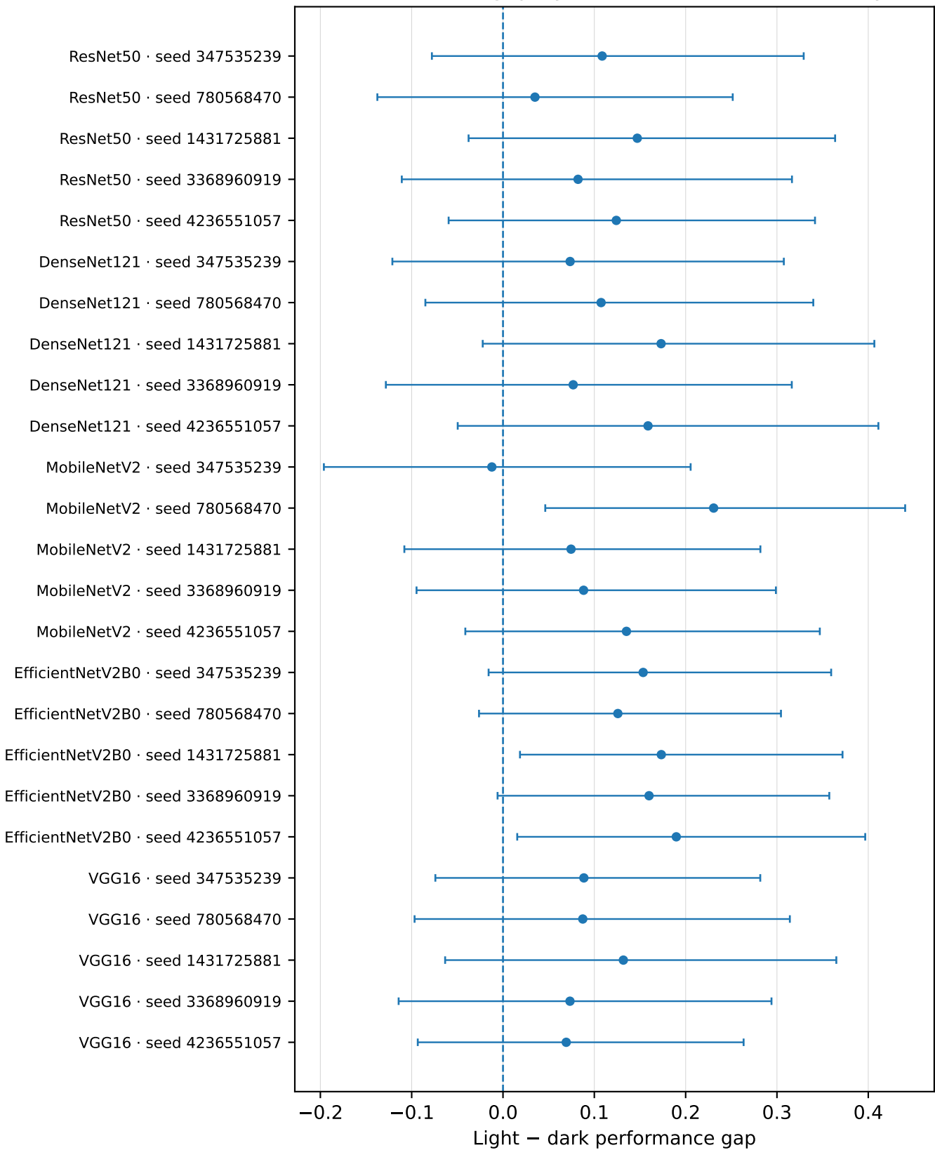
BOSQUE F1-score gap by locked architecture-seed system
