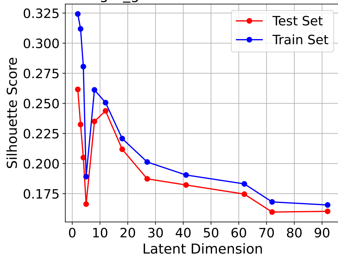
target_gene — Euclidean distance
