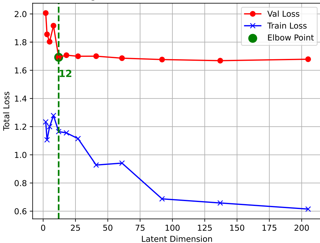
Training and Validation Loss vs Latent Dimension
