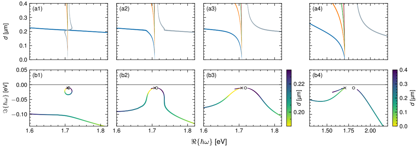
Oscillator Strength Scaling: 0.025
