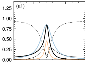
Oscillator Strength Scaling: 0.025
