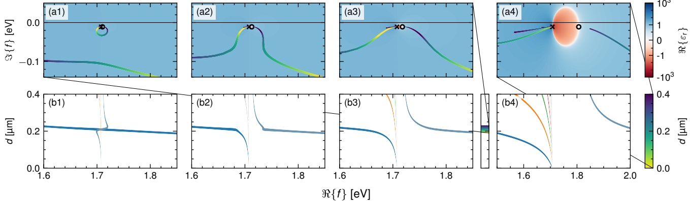
Oscillator Strength Scaling: 0.025
