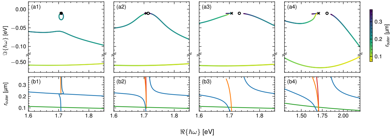
Oscillator Strength Scaling: 0.01
