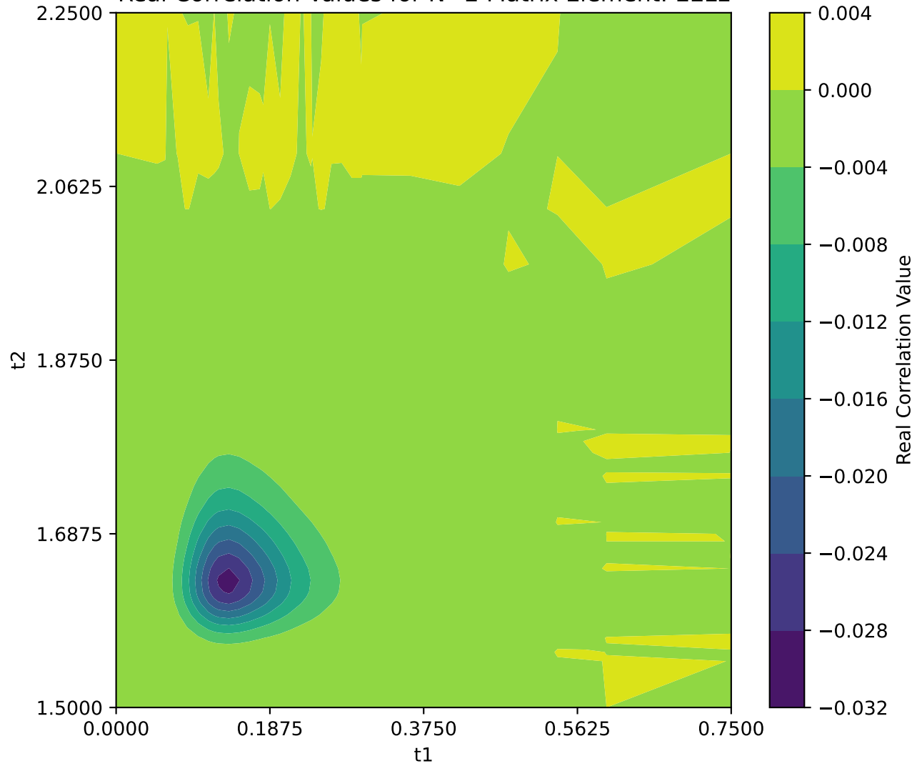
Real Correlation Values for N=2 Matrix Element: EELL
