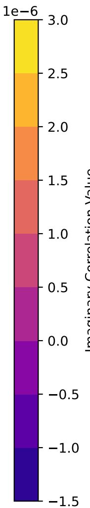
Imaginary Correlation Values for N=2 Matrix Element: ELEL
