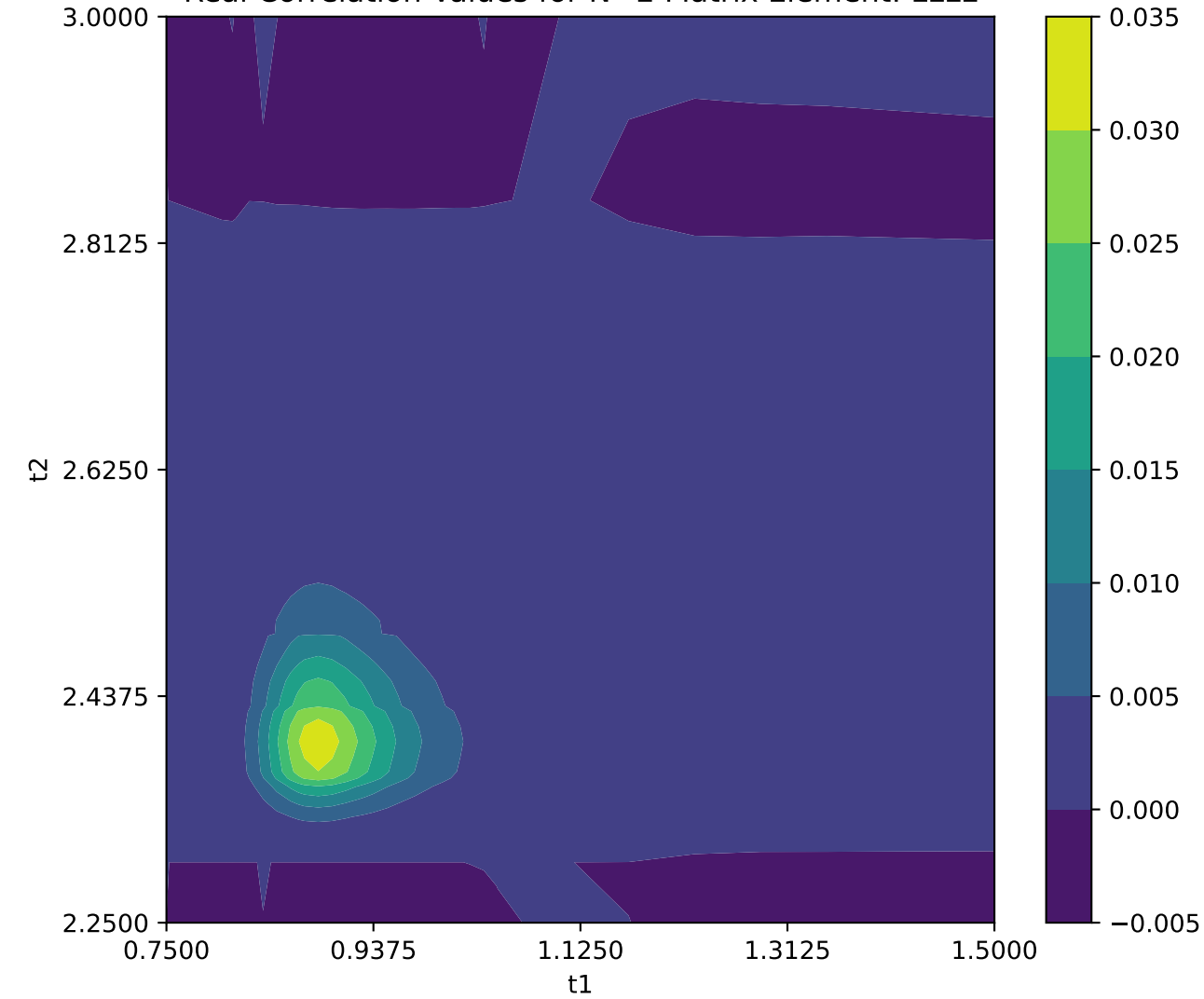
Real Correlation Values for N=2 Matrix Element: LLLL
