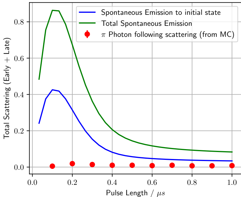
Scattering Rates vs Driving Pulse Length
