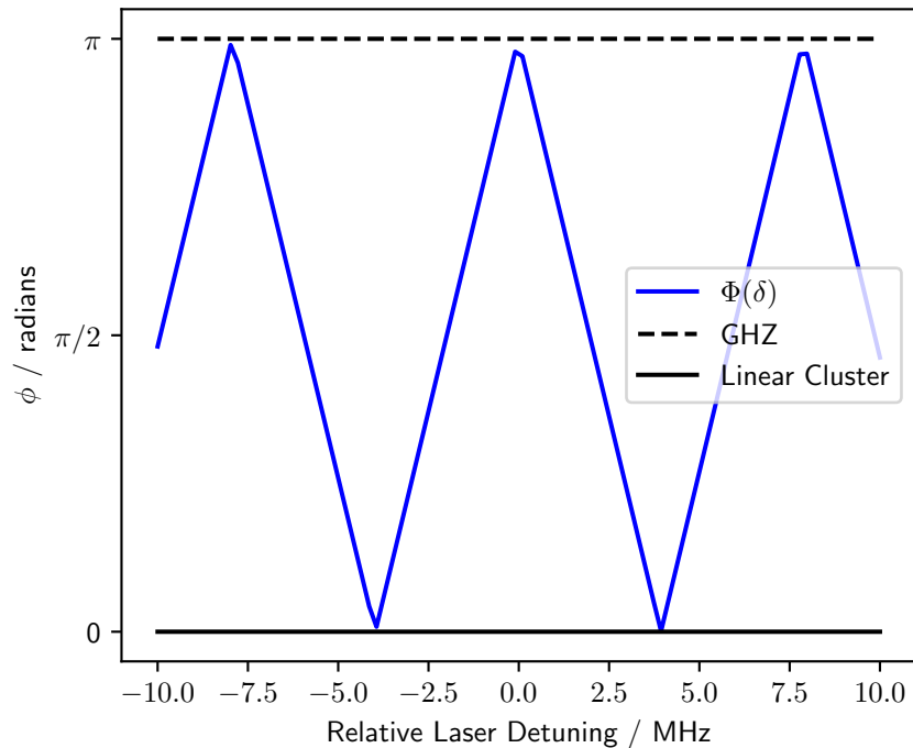
Evolution of \Phi with laser detuning for Rotation 7
