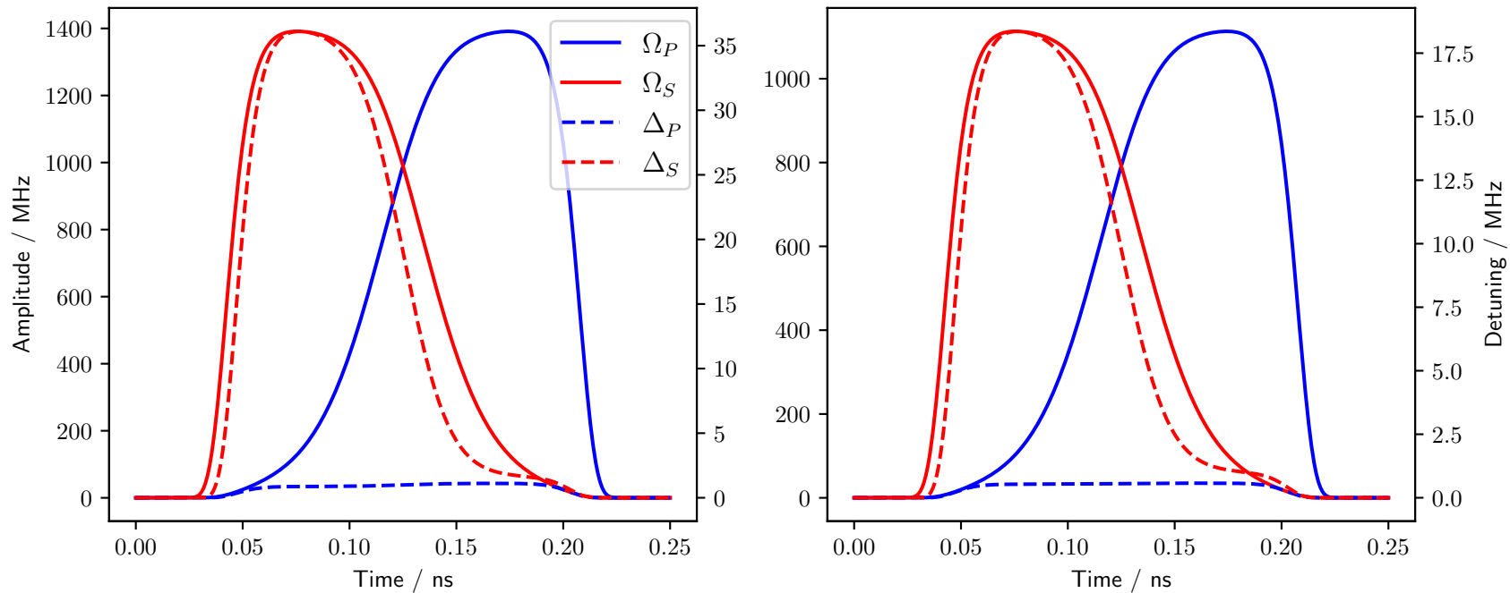
Masked STIRAP rotations 5 and 7 with frequency chirp
