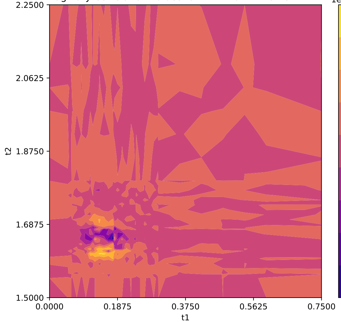
Imaginary Correlation Values for N=2 Matrix Element: ELEL
