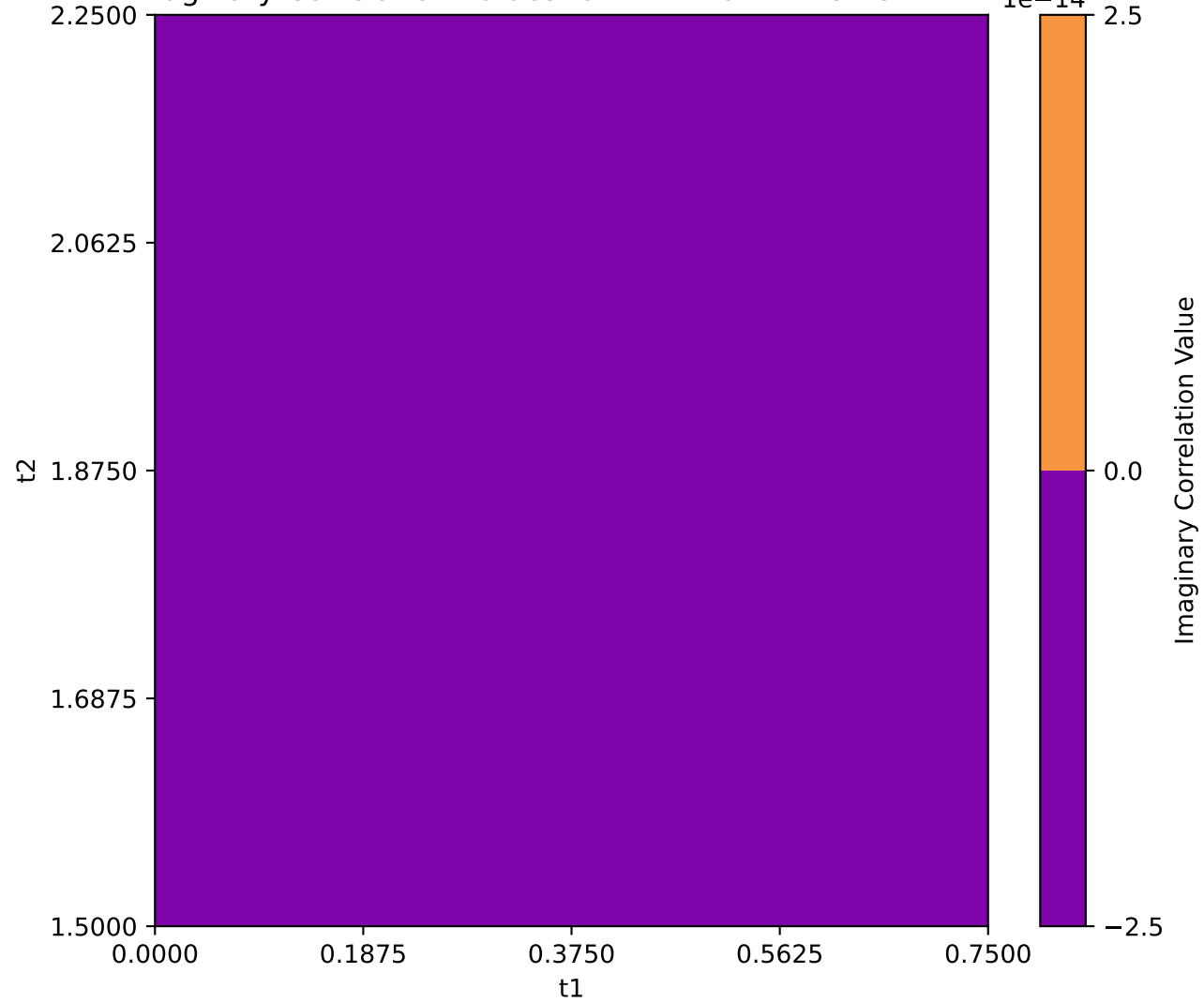
Imaginary Correlation Values for N=2 Matrix Element: EEEE
