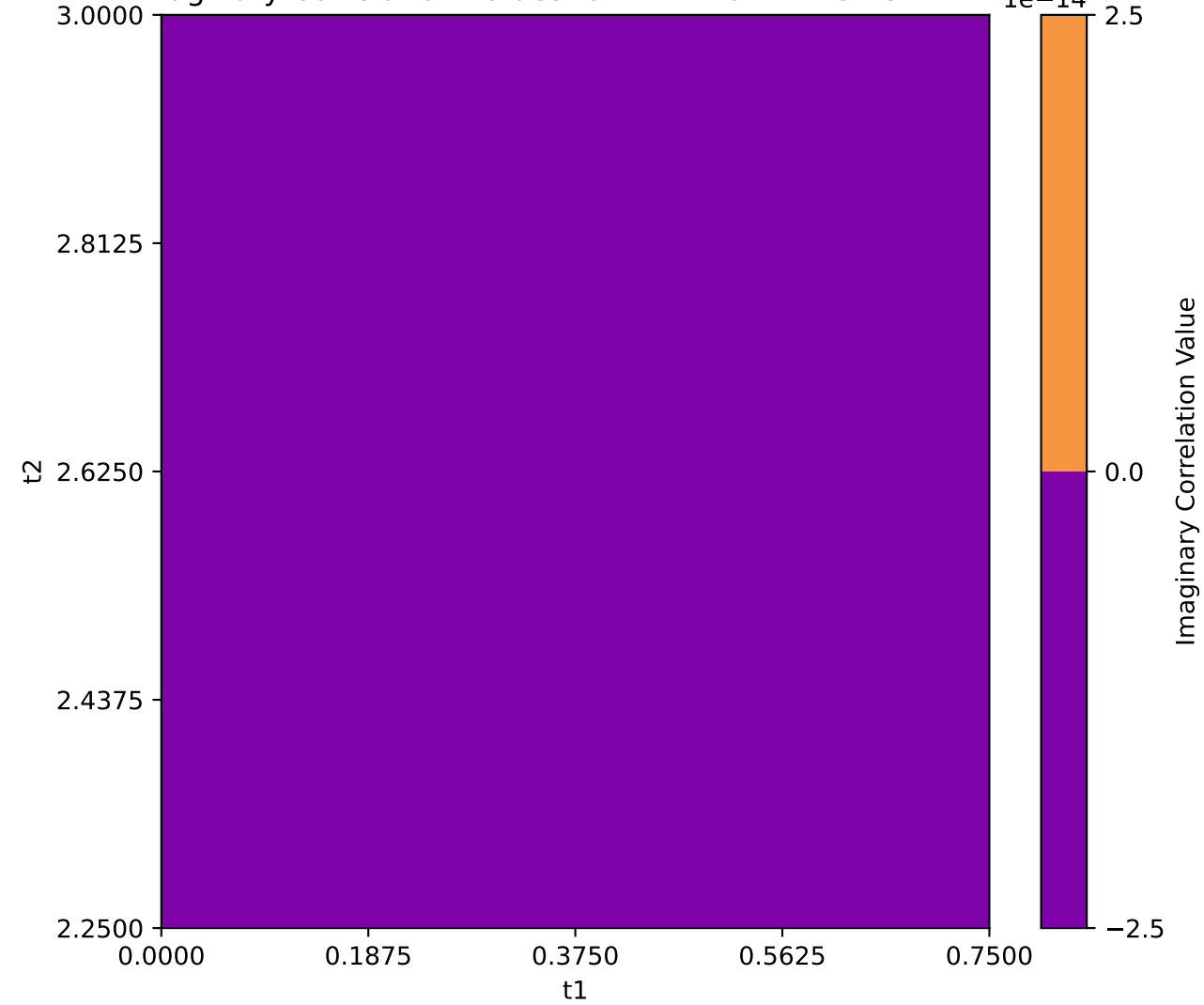
Imaginary Correlation Values for N=2 Matrix Element: ELLE
