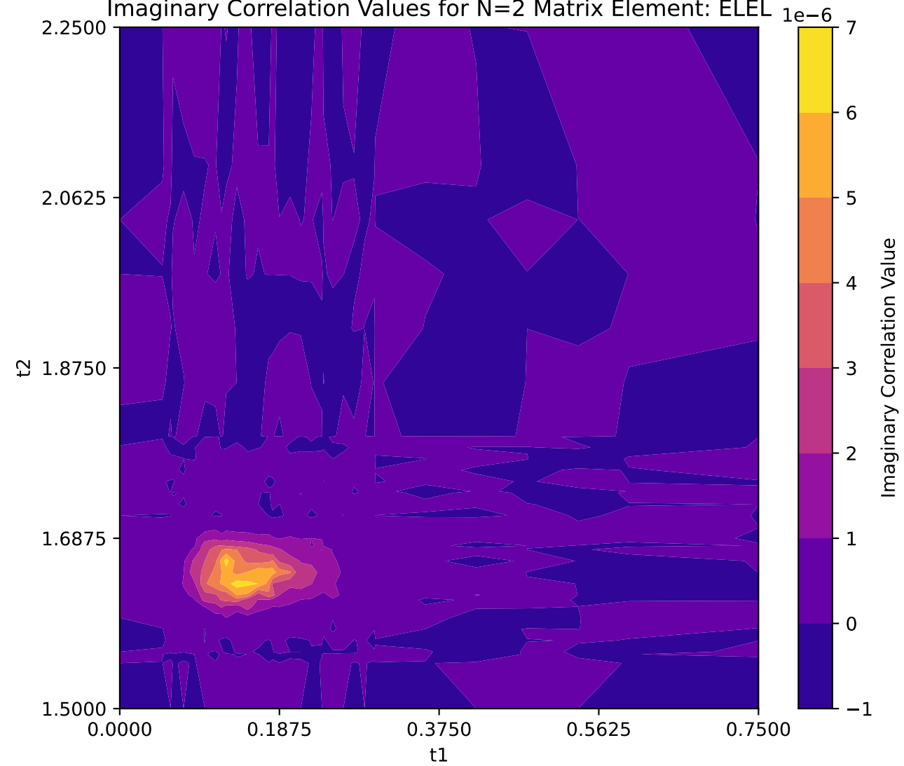
Imaginary Correlation Values for N=2 Matrix Element: ELEL
