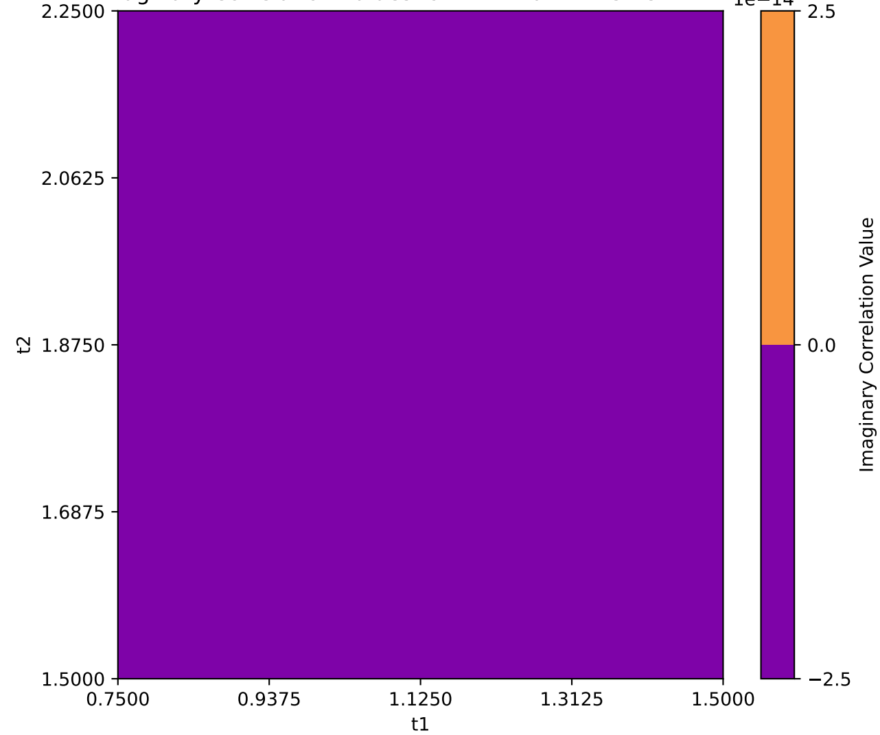
Imaginary Correlation Values for N=2 Matrix Element: LEEL
