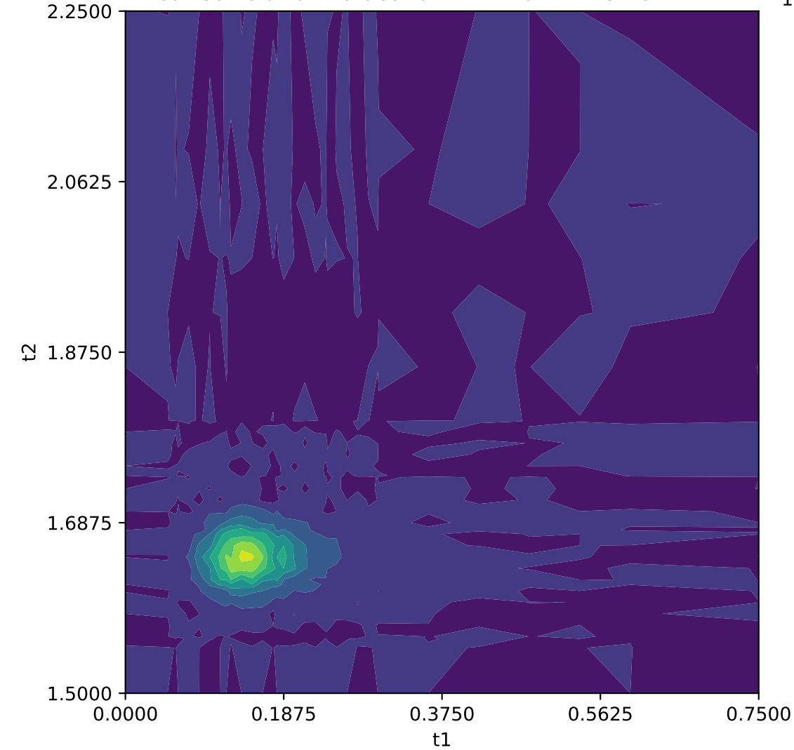
Real Correlation Values for N=2 Matrix Element: ELEL
