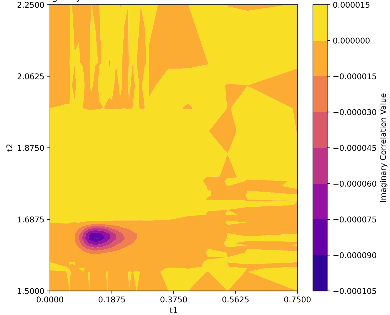
Imaginary Correlation Values for N=2 Matrix Element: ELEL
