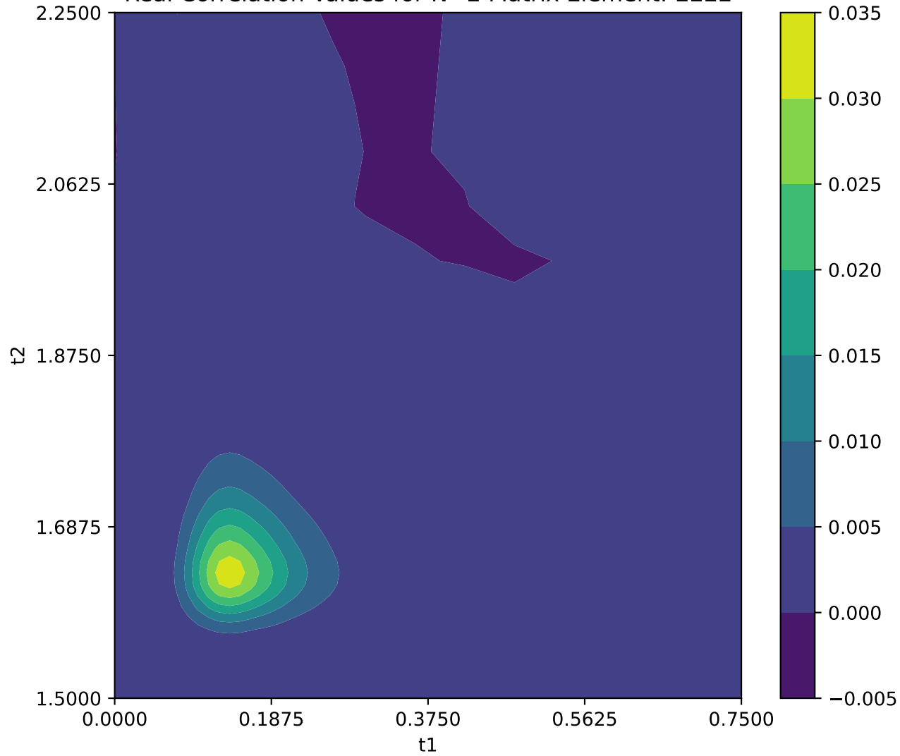
Real Correlation Values for N=2 Matrix Element: EEEE
