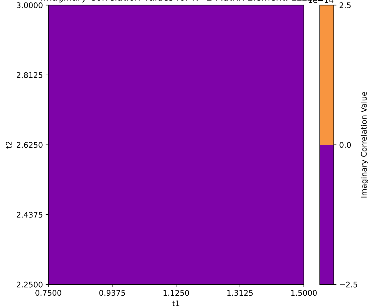
Imaginary Correlation Values for N=2 Matrix Element: LLLL
