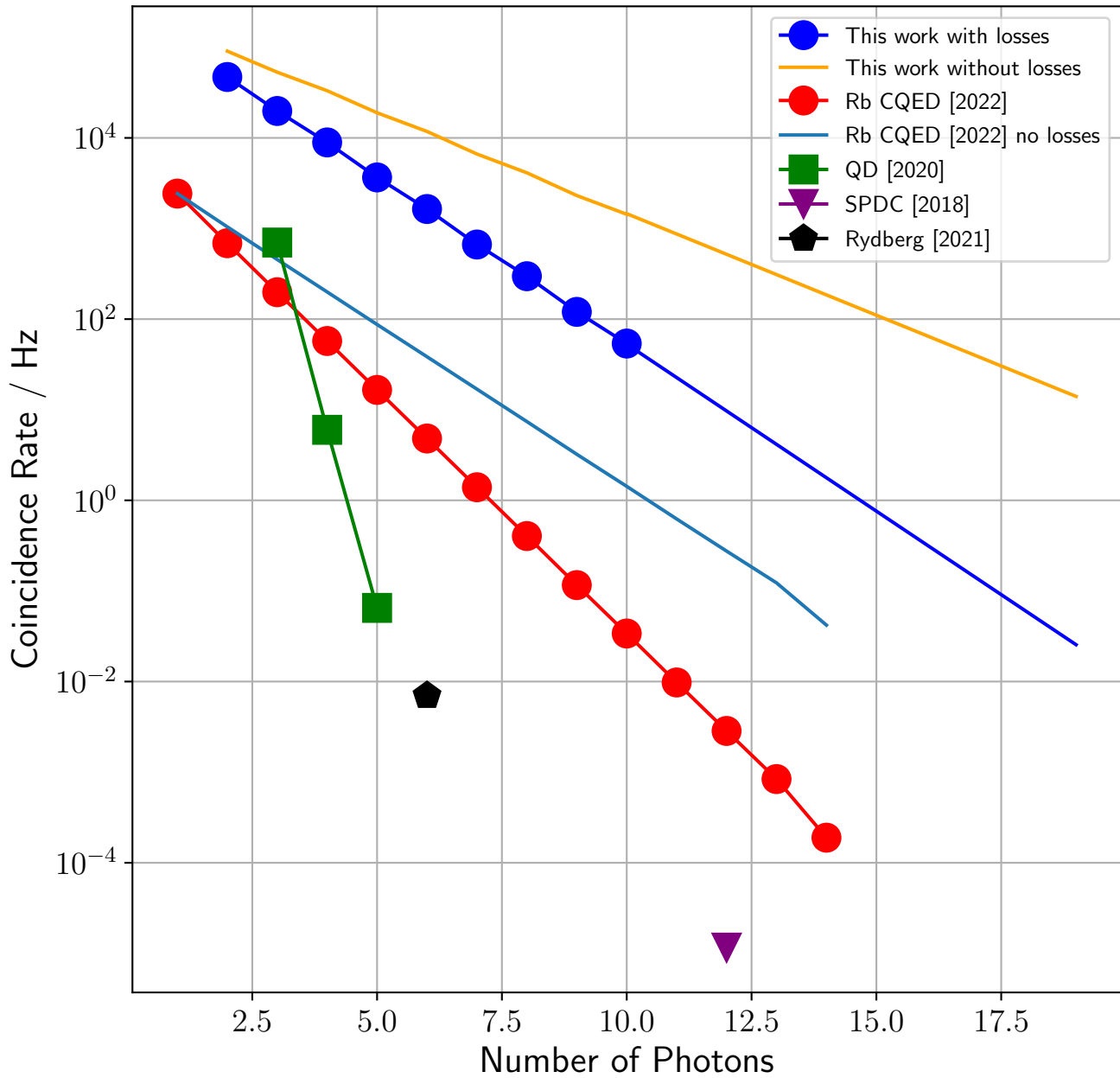
Coincidence Rate vs Number of Photons in GHZ State
