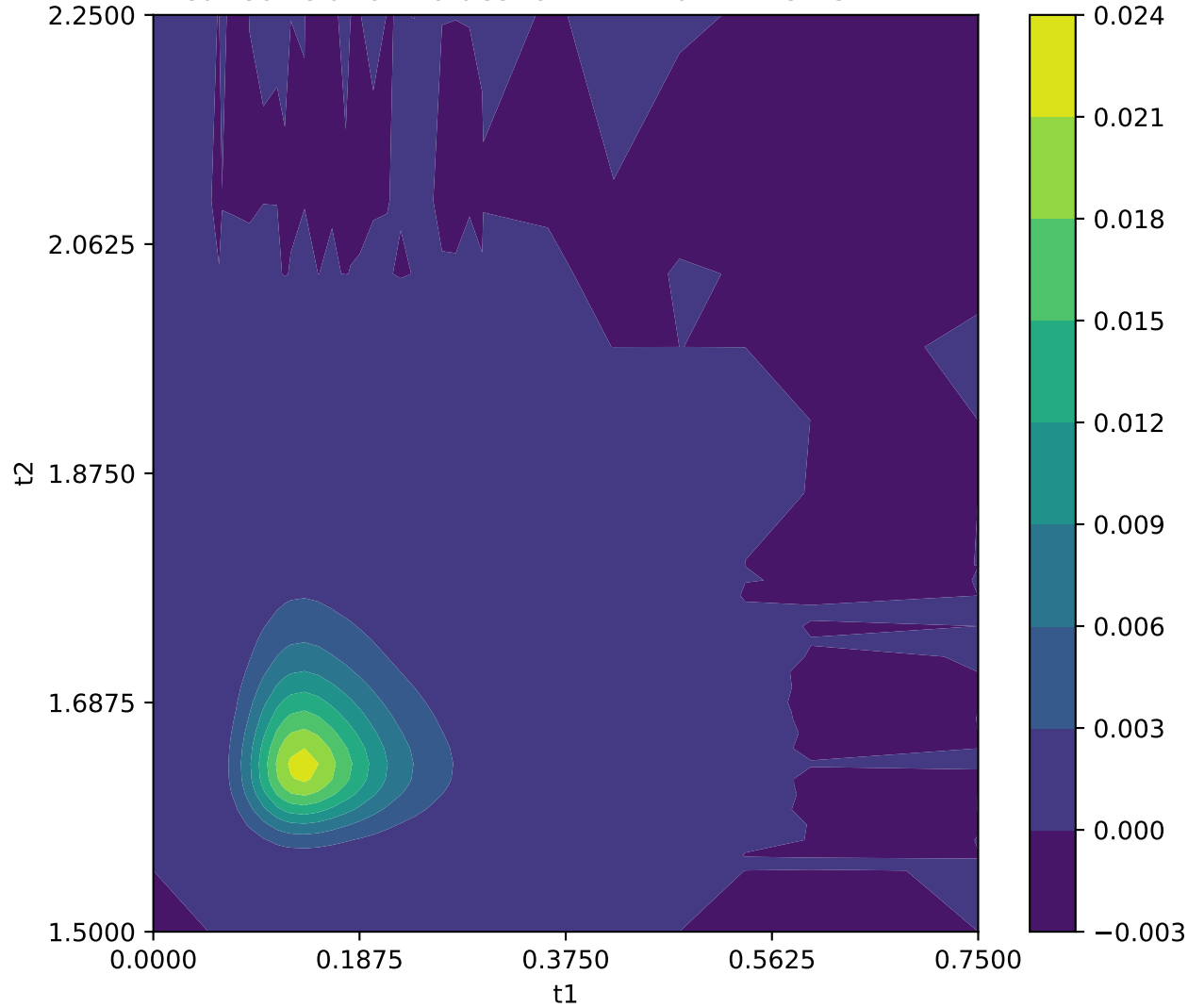
Real Correlation Values for N=2 Matrix Element: EELL
