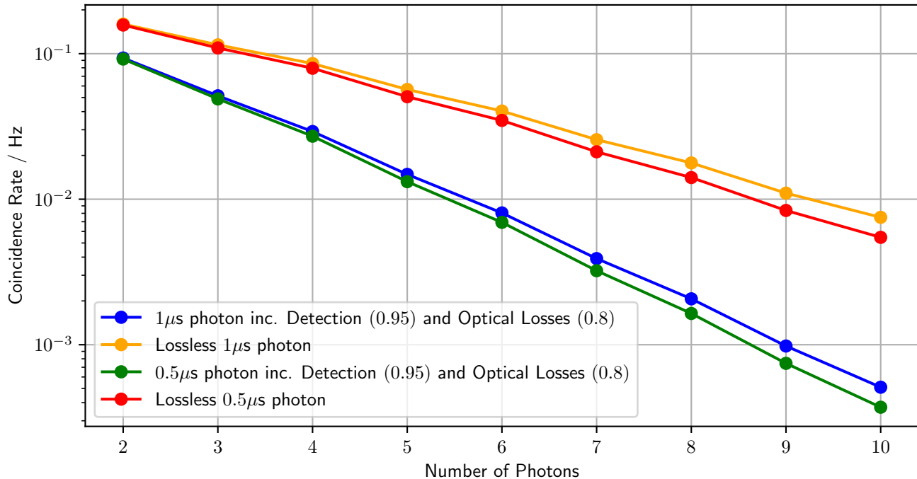
Coincidence Rate vs Number of Photons in GHZ State
