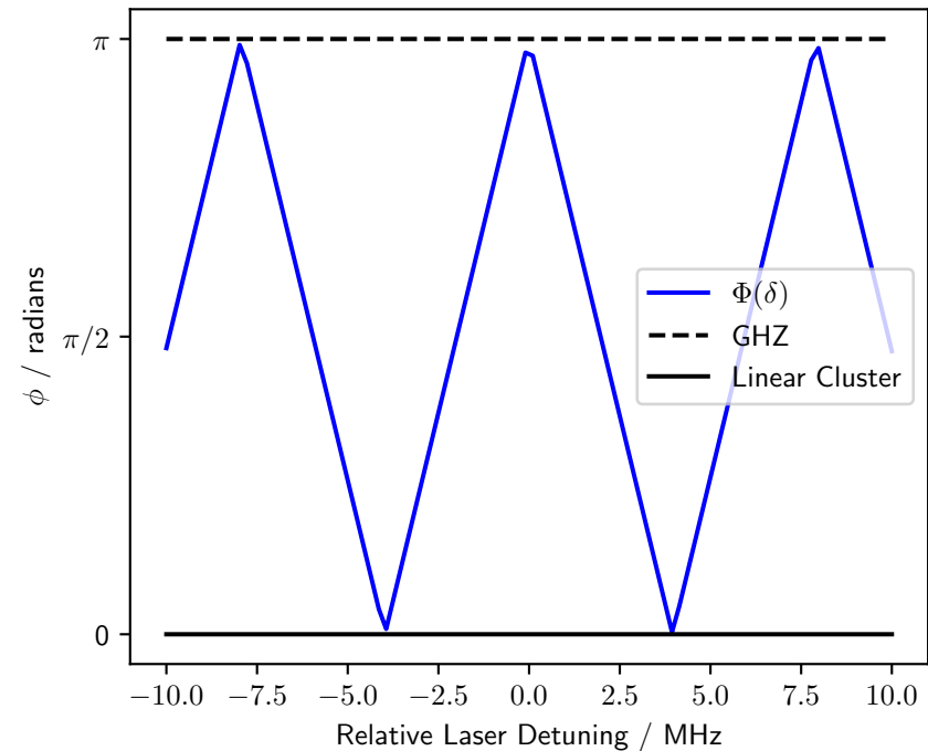
Evolution of \Phi with laser detuning for Rotation 5
