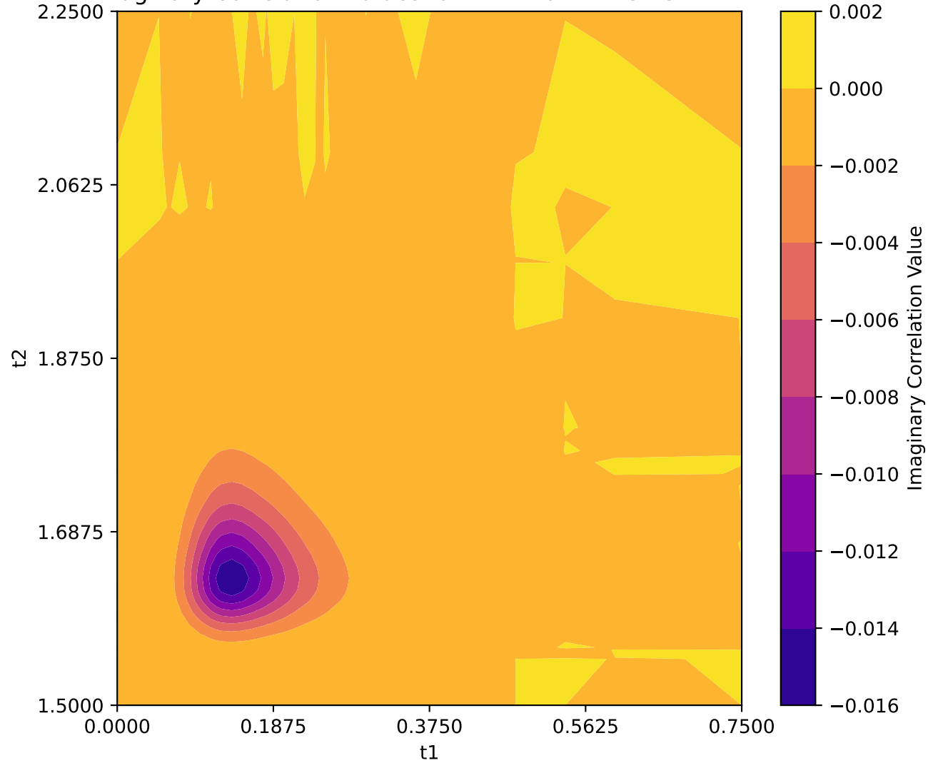
Imaginary Correlation Values for N=2 Matrix Element: EELL
