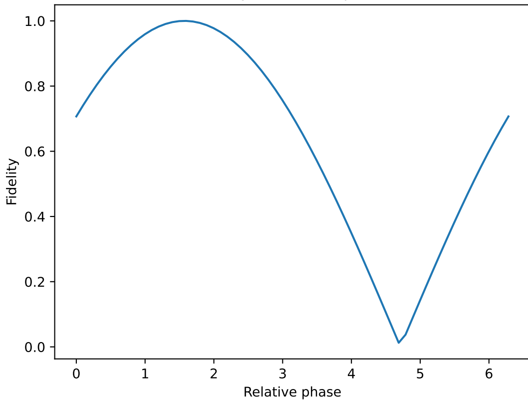
Fidelity vs relative phase
