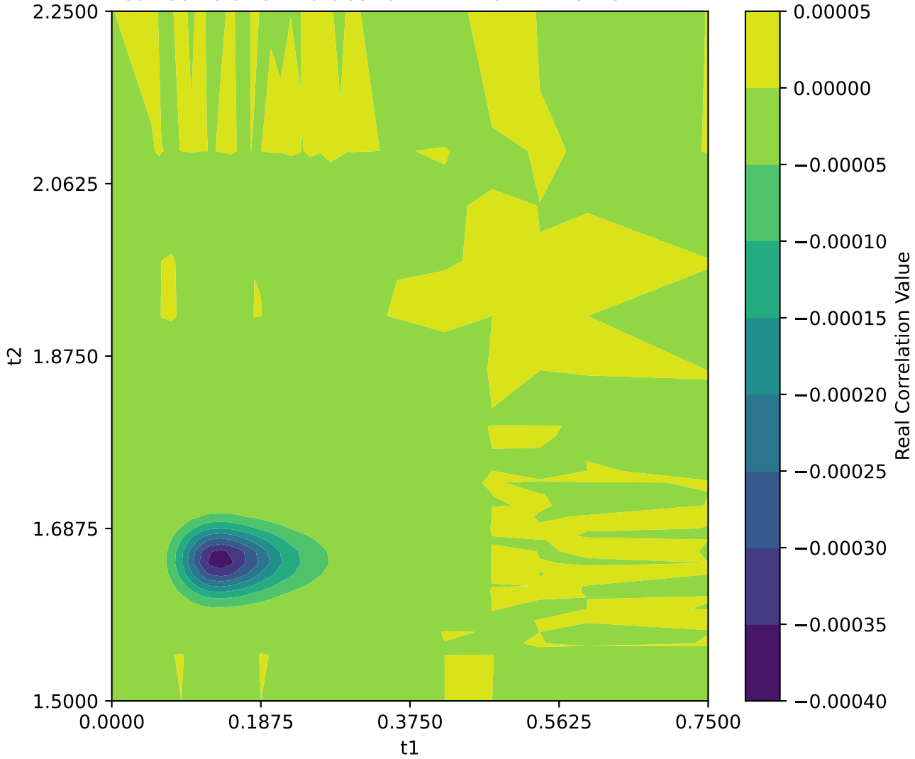
Real Correlation Values for N=2 Matrix Element: ELEL
