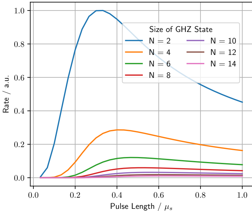
Expected Photon Coincidences for different N at \Omega L=50.0
