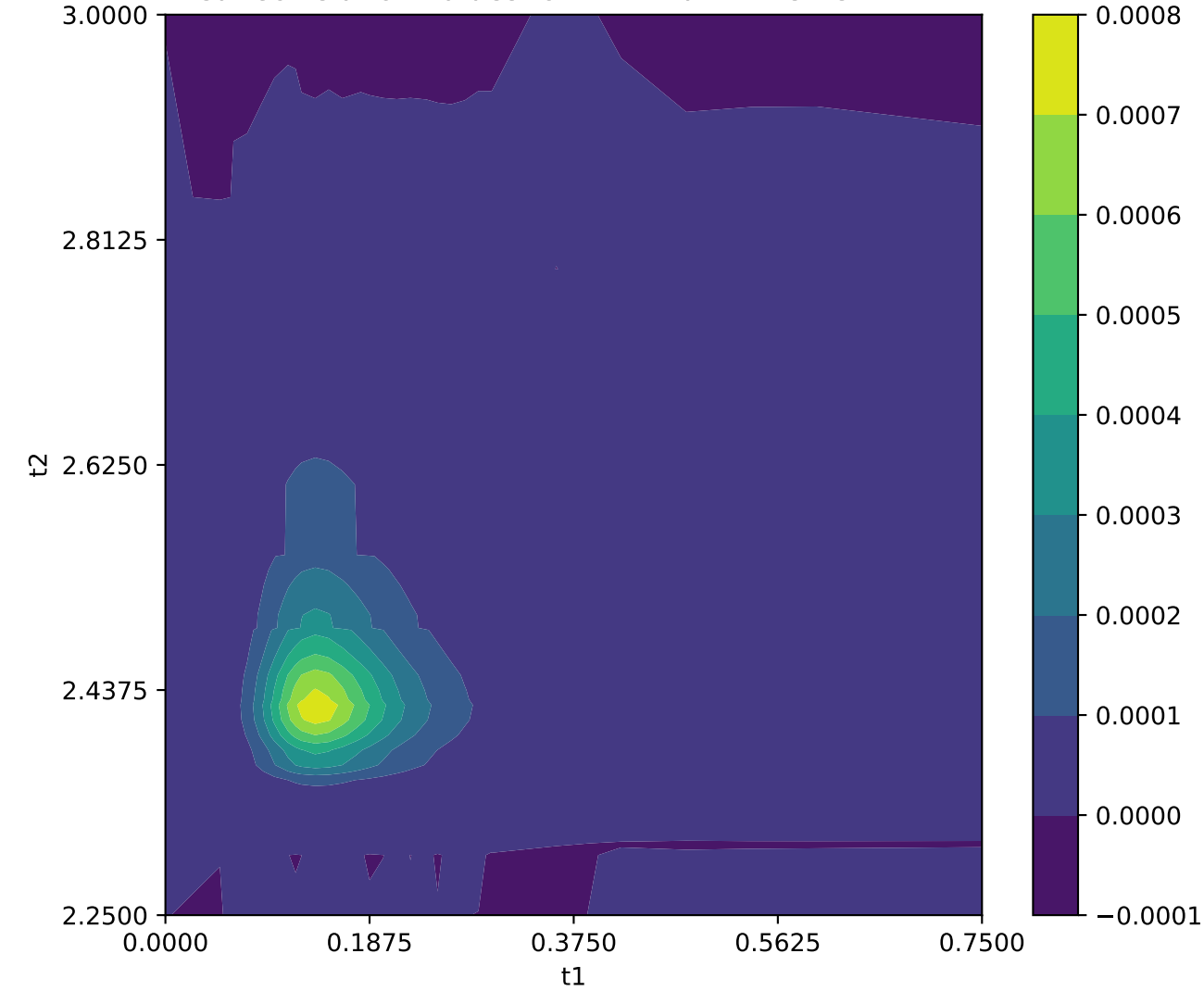
Real Correlation Values for N=2 Matrix Element: ELLE
