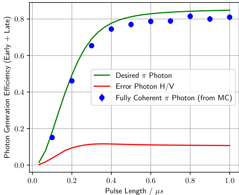
Length of Driving Pulse vs Expected Photon Rate/ qubit at \Omega L=50
