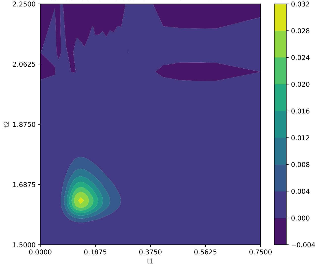
Real Correlation Values for N=2 Matrix Element: EEEE
