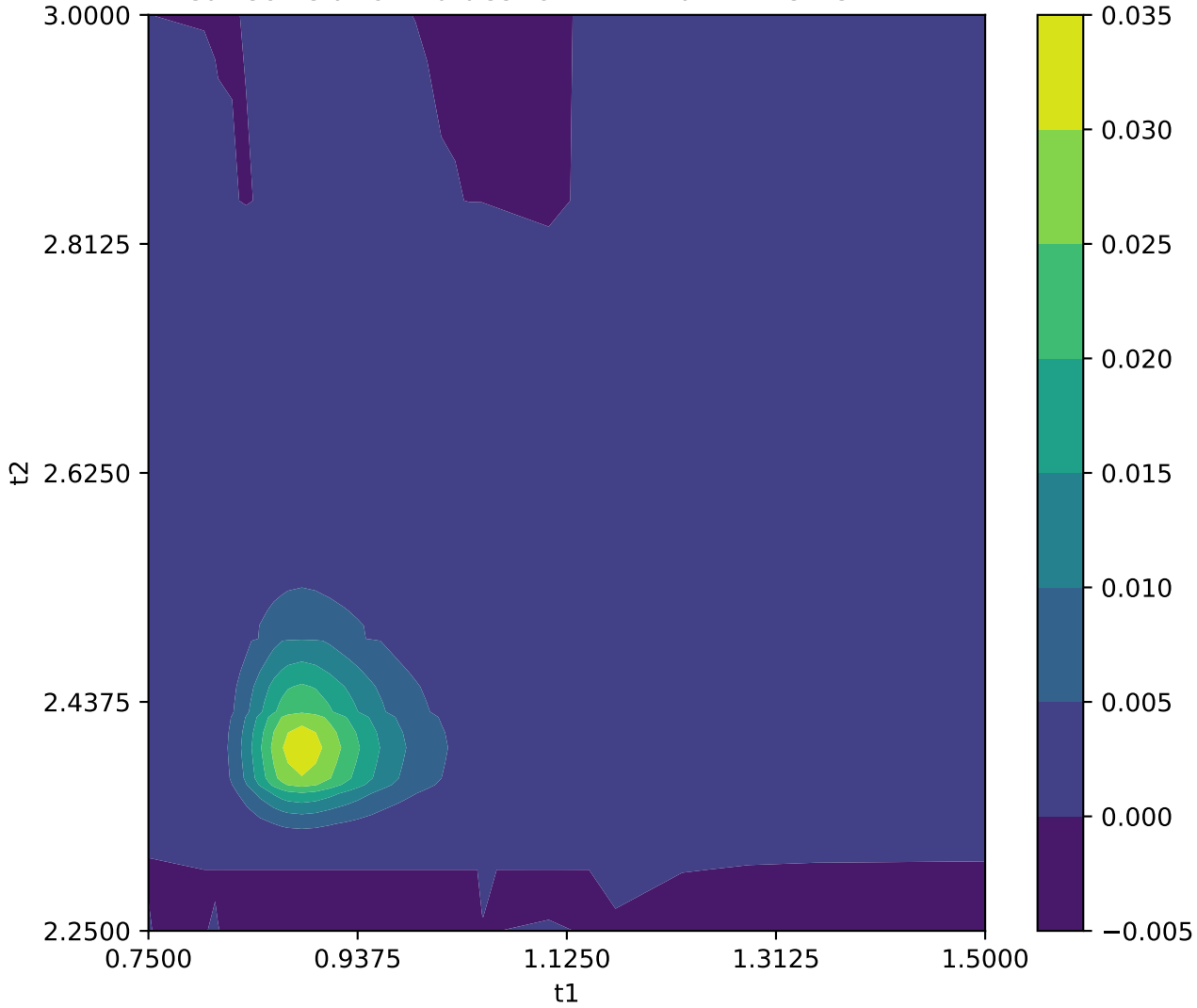
Real Correlation Values for N=2 Matrix Element: LLLL
