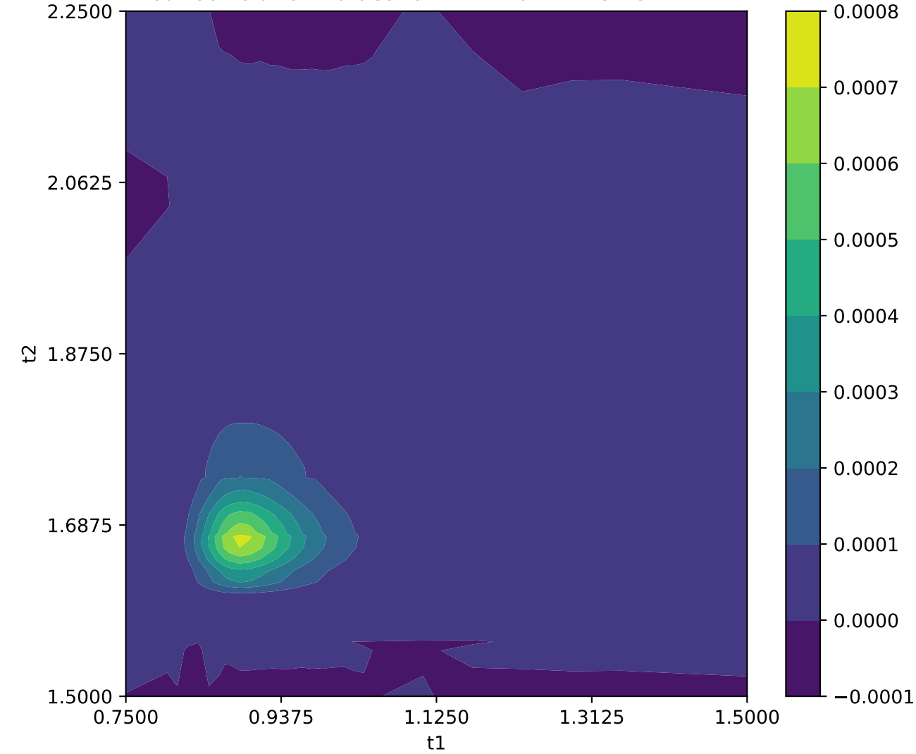
Real Correlation Values for N=2 Matrix Element: LEEL
