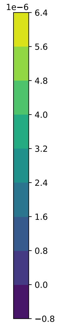
Real Correlation Values for N=2 Matrix Element: ELEL
