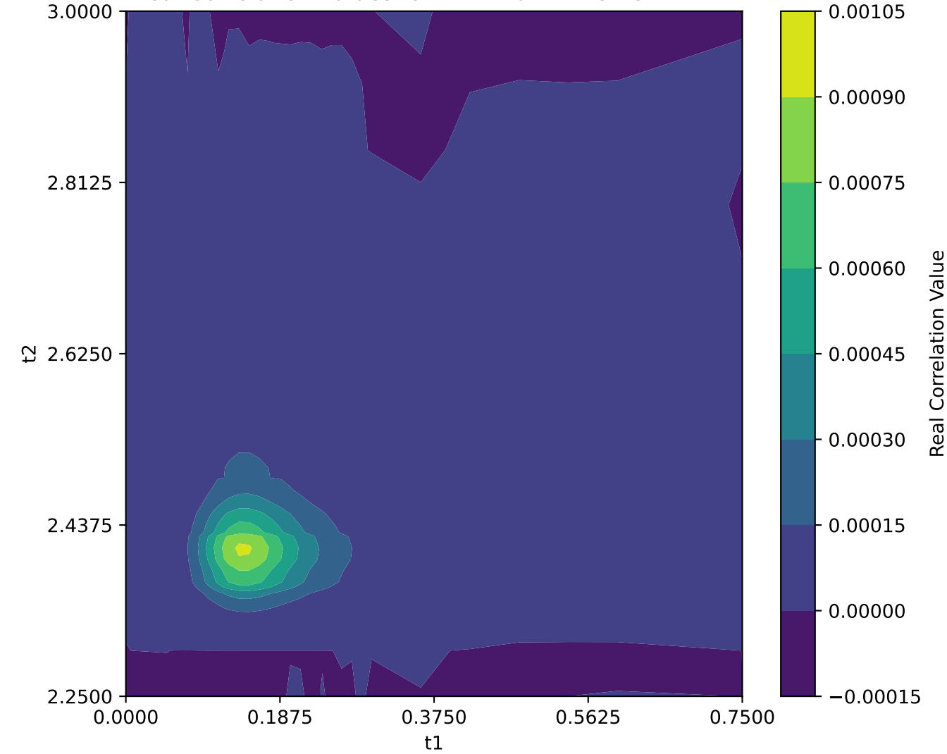
Real Correlation Values for N=2 Matrix Element: ELLE
