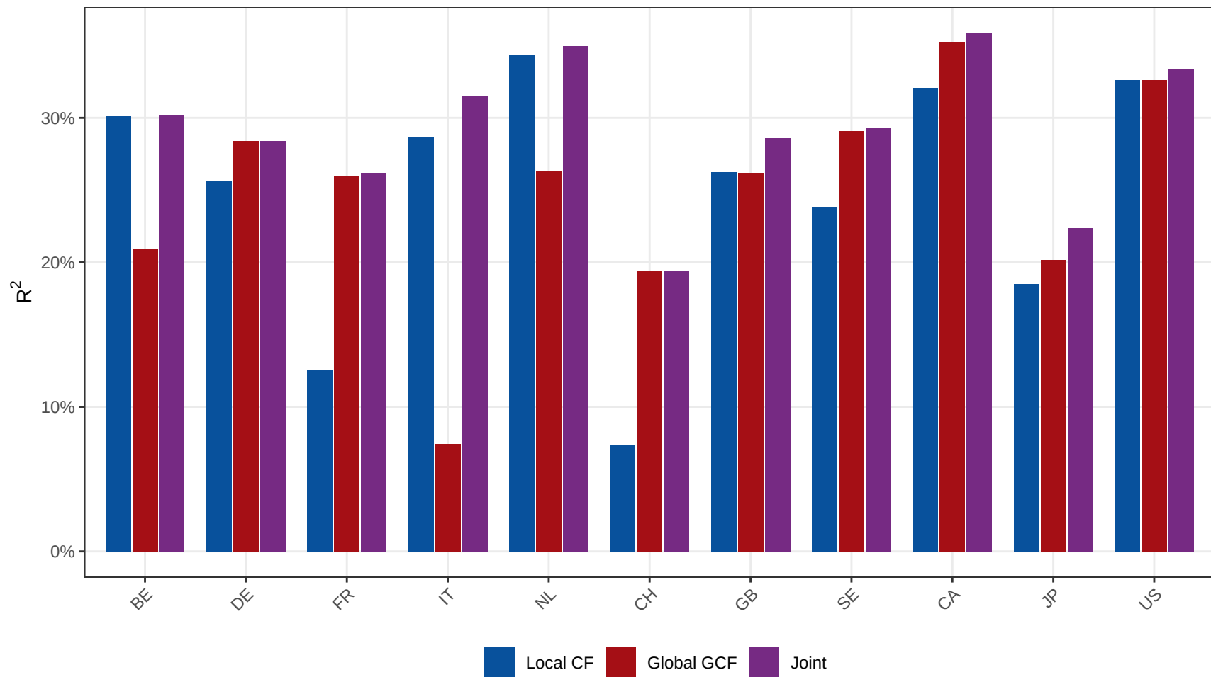
Phase II: in-sample R^2 ladder per country
