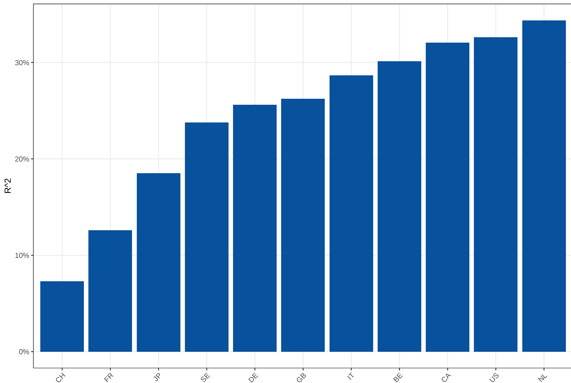
In-sample R^2 of rx sim CF by country
