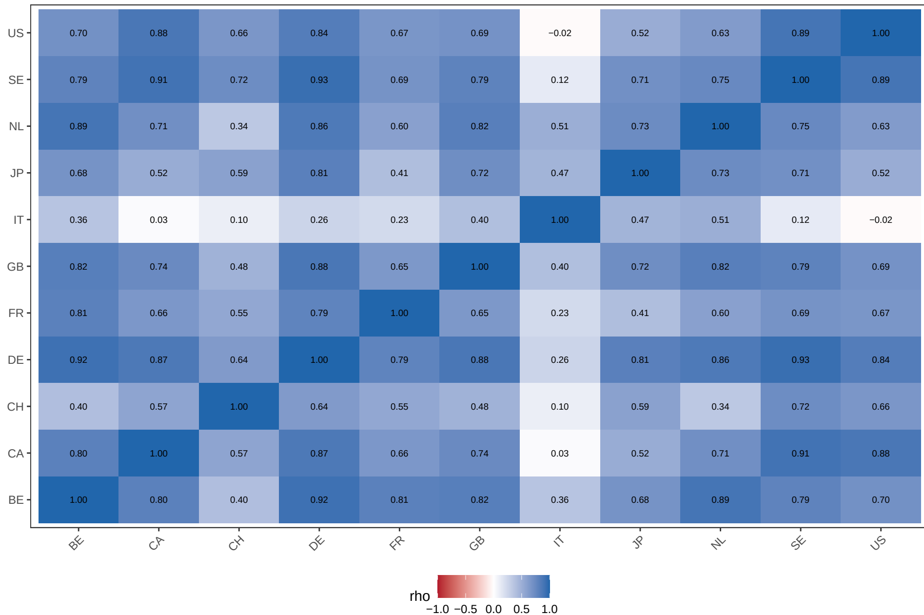
Pairwise correlation of local cycle factors
