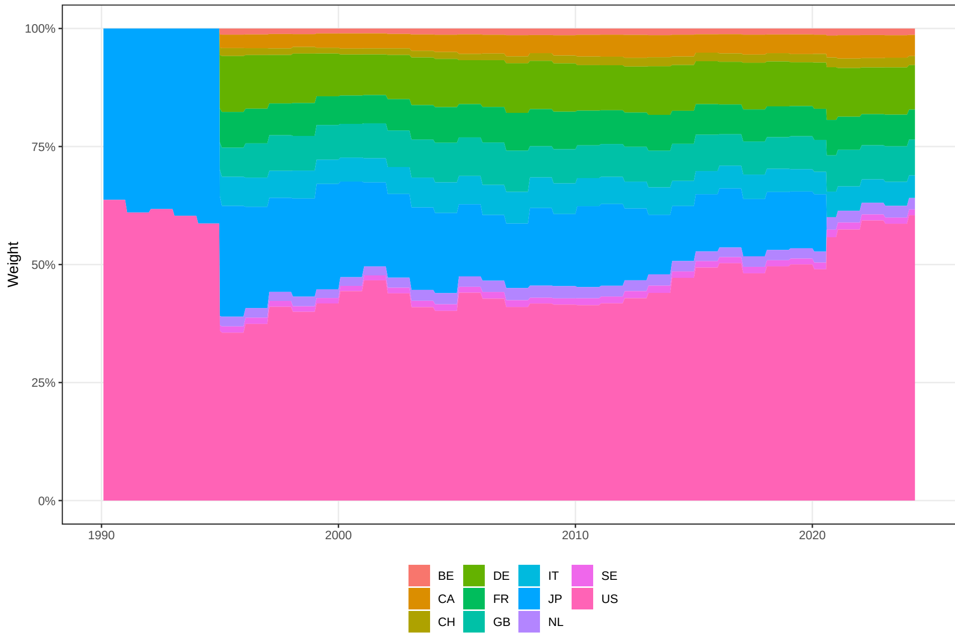
GDP weights w_{i,t} across the panel (eq 8)
