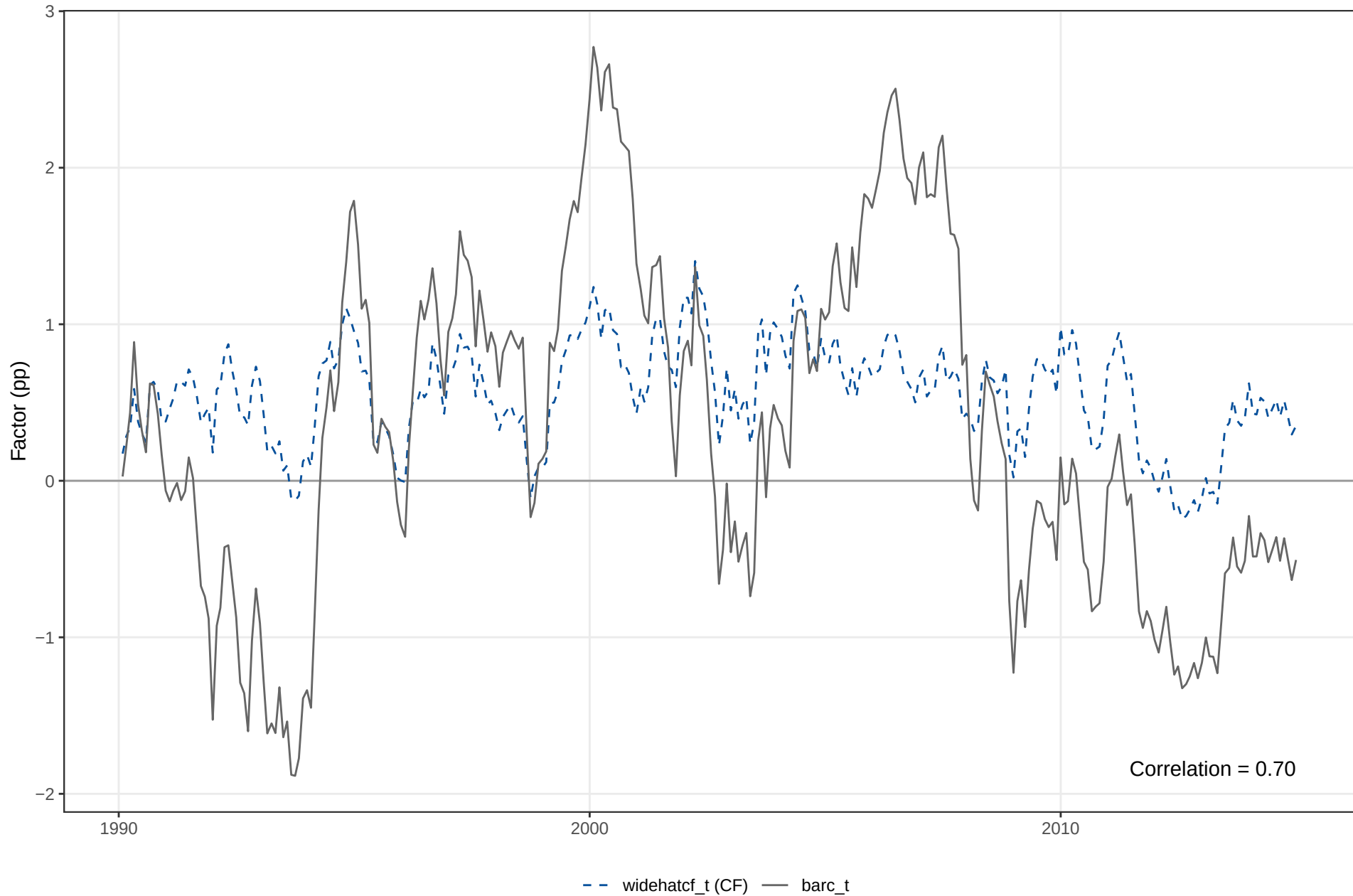
US: return-forecasting factor and average cycle (CP-2015 Fig. 2)
