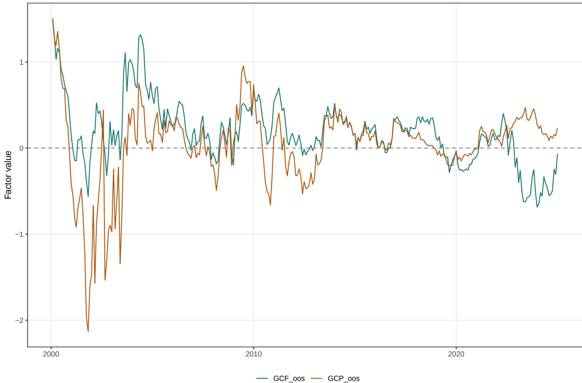
OOS global factor: GCF_oos vs GCP_oos (fully recursive)
