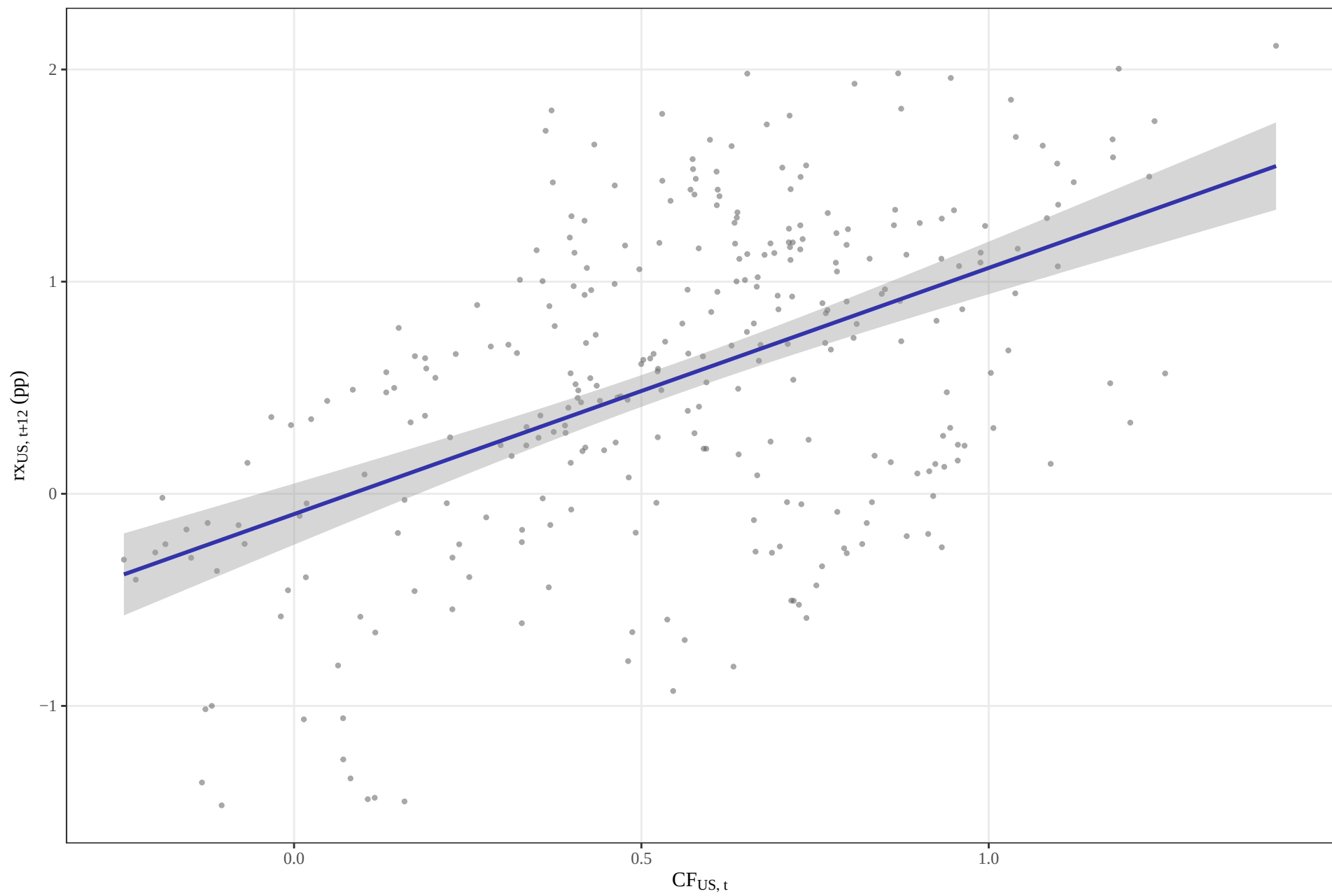
US: excess return vs cycle factor (CP-2015 predictability)
