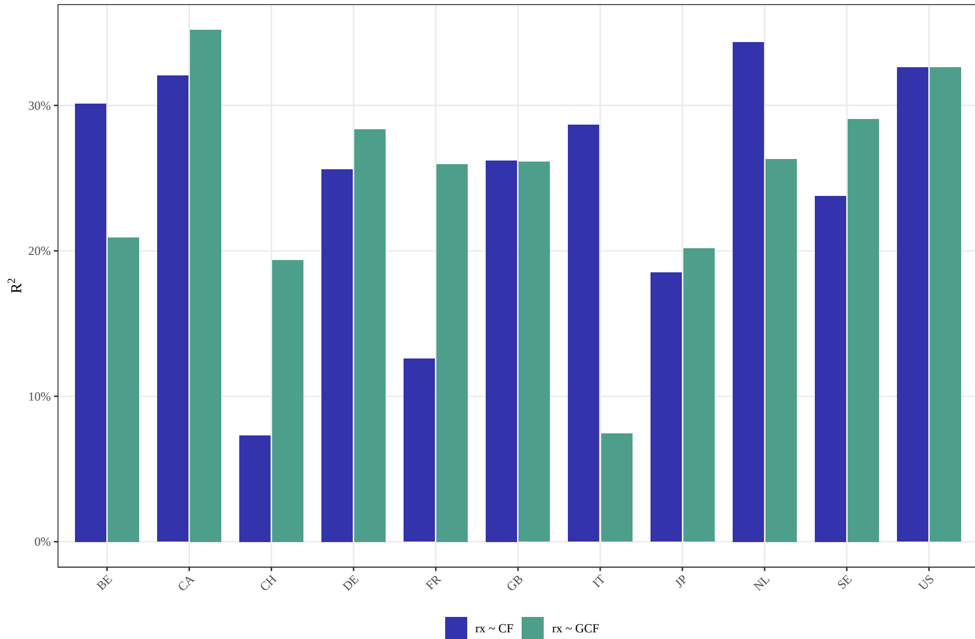
In-sample R^2 : local CF vs global GCF
