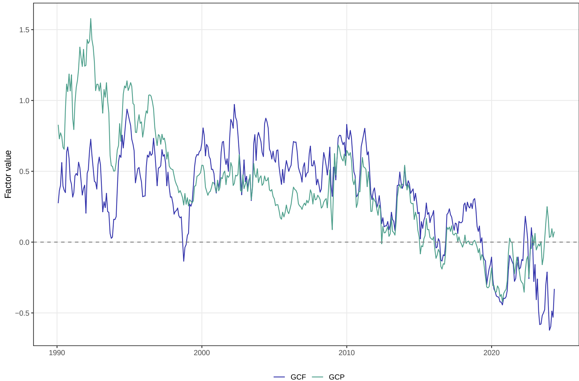
Global factor: GCF vs GCP (in-sample)
