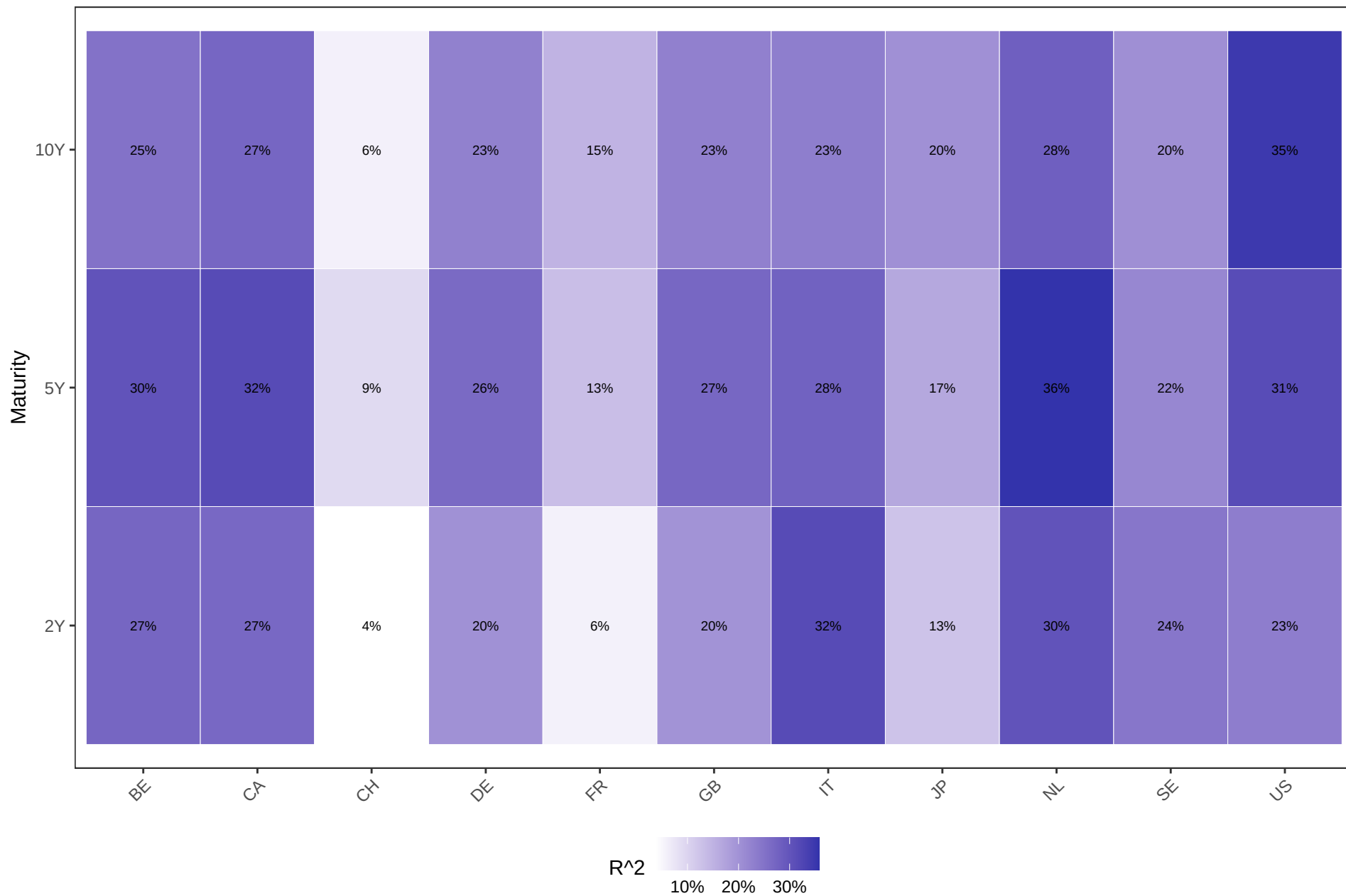
In-sample R^2 of rx^{(n)} sim CF by country and maturity
