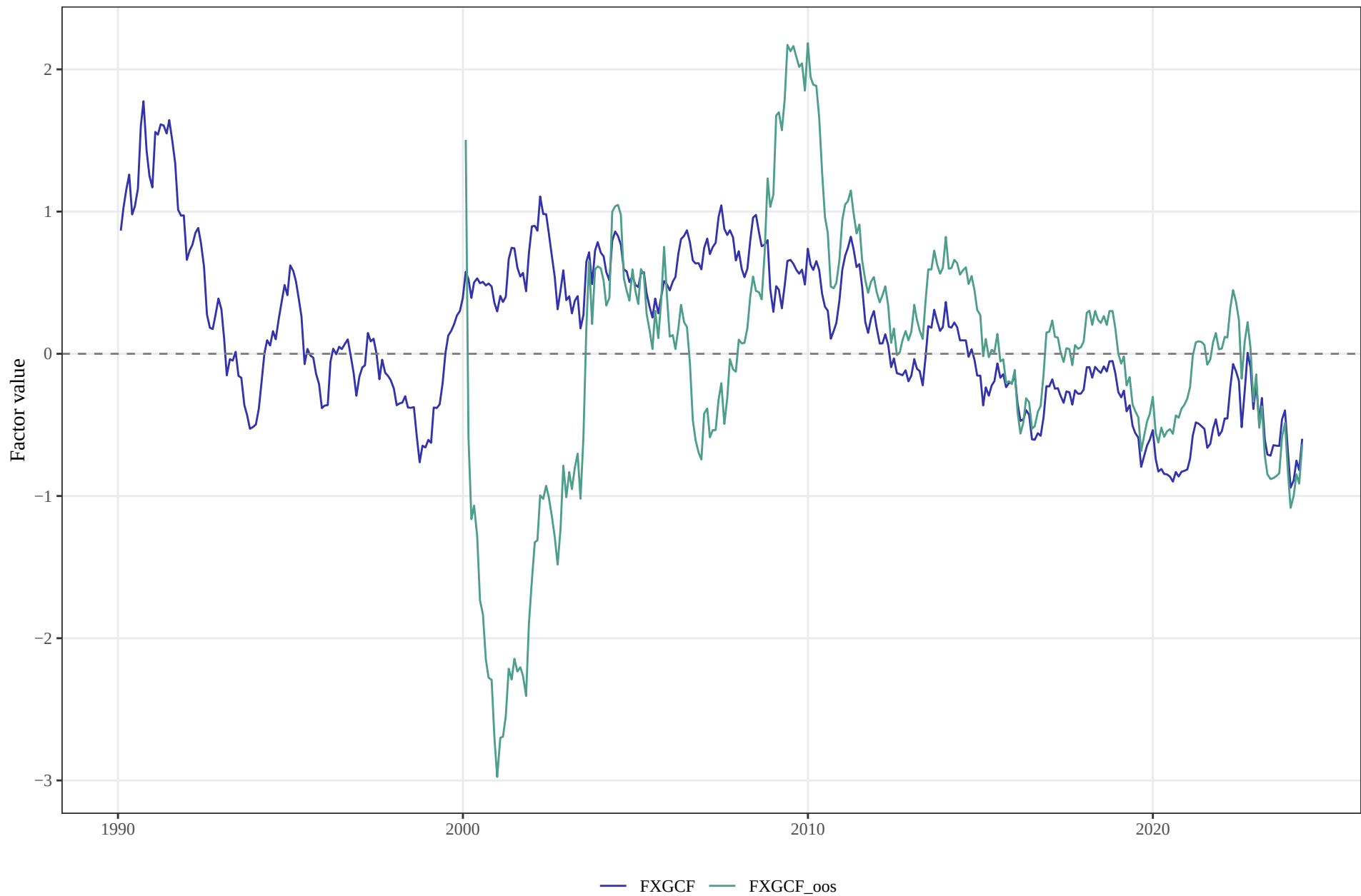
FX-adjusted GCF: full-sample FXGCF vs fully-recursive FXGCF_oos
