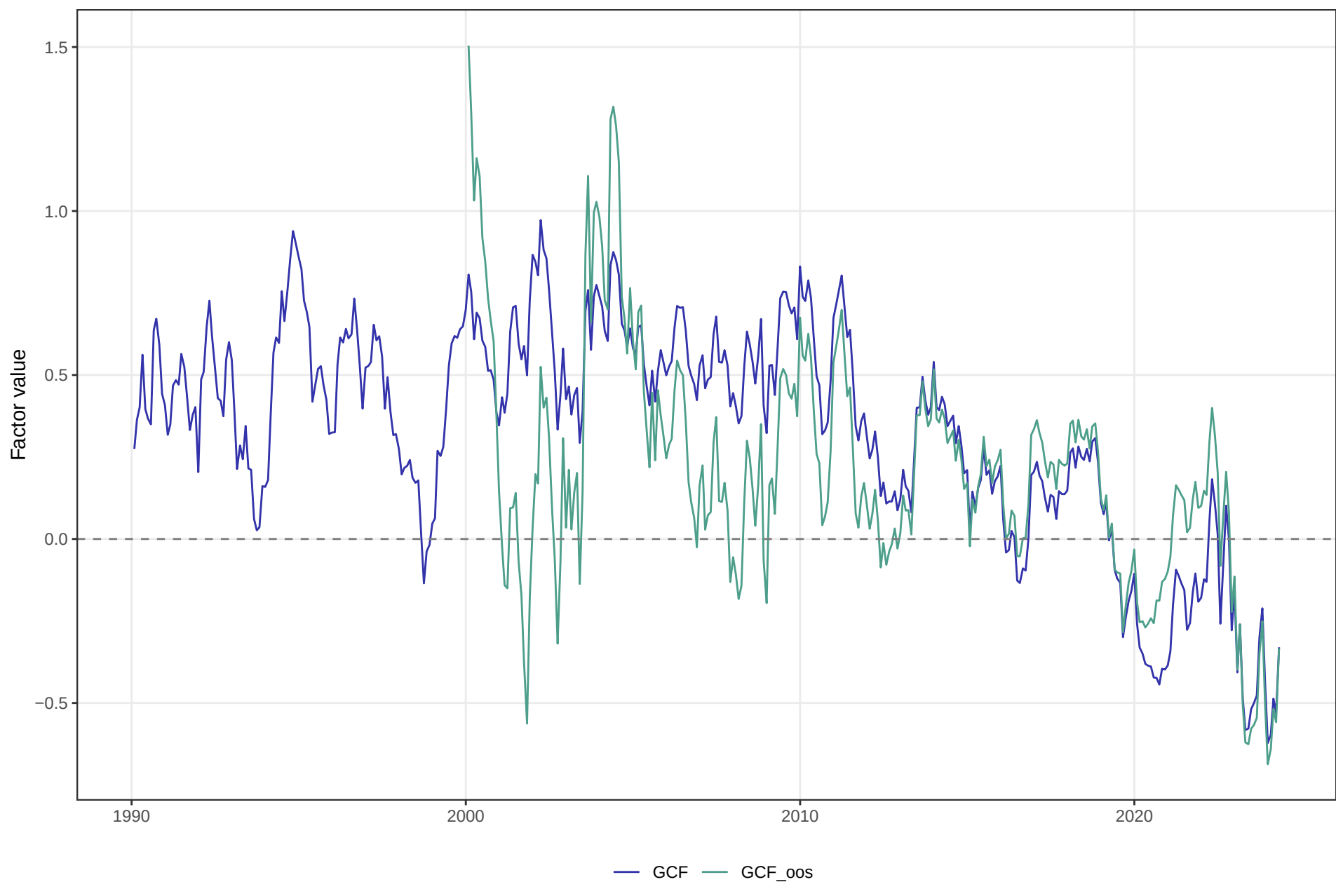
Global cycle factor: full-sample GCF vs fully-recursive GCF_oos
