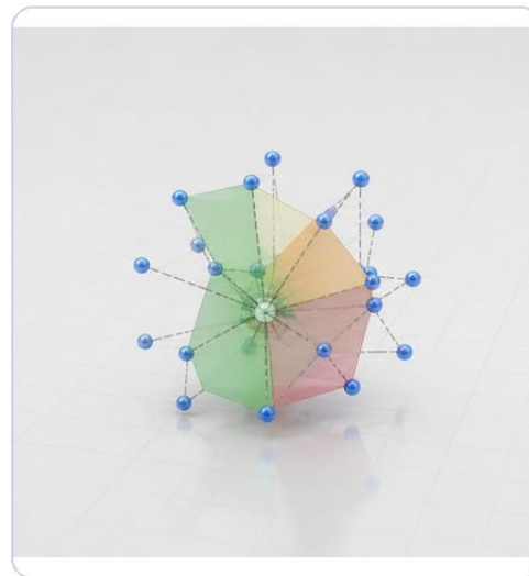
DIAGNOSTIC LABEL
