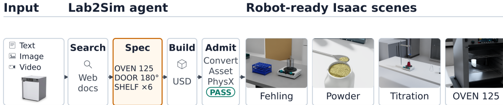
Figure 1: Text, image, and video form one request interface. Lab2Sim searches manufacturer evidence, writes an asset specification, builds articulated USD with a Blender skill (Blender Foundation, 2024), and admits it through ConvertAsset. Hunyuan3D is an optional geometry frontend (Tencent Hunyuan3D, 2025). Right: Fehling, powder, titration, and OVEN 125 Isaac scenes the agent delivered from independent requests.
