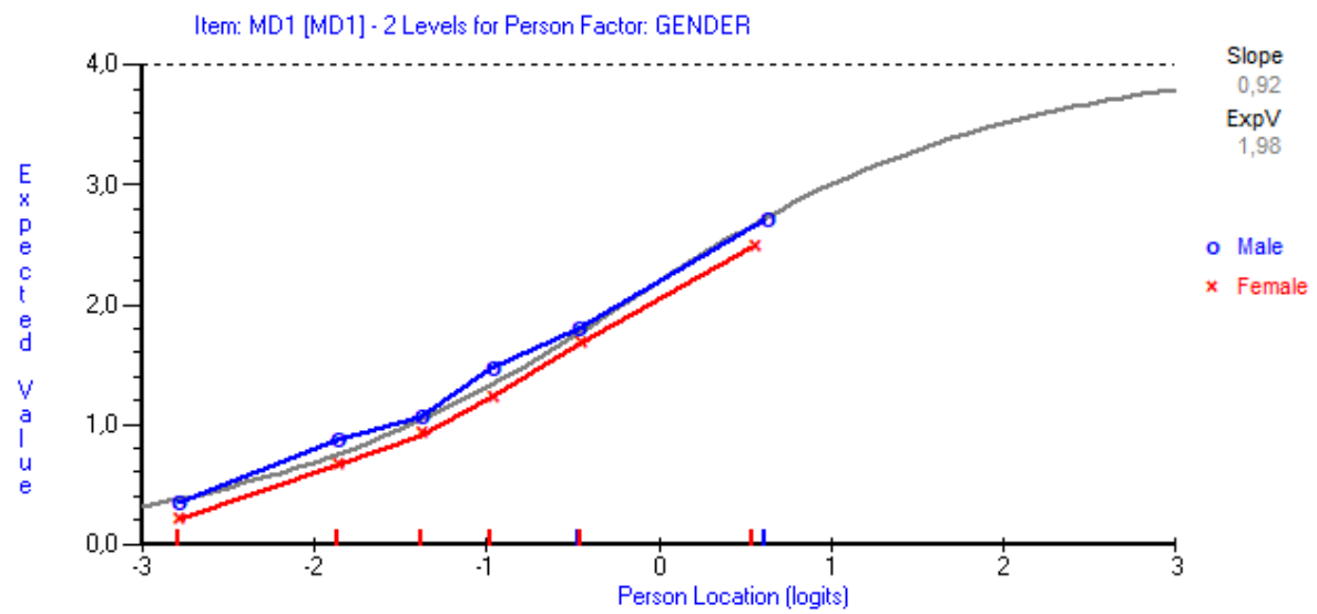
Fig 3. The item characteristic curve of item MD1 (I struggle to find any enthusiasm for my work) for women and men in a sample from Germany (n=1073).
