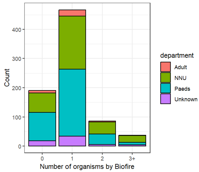
S2 Fig. Number of organisms identified by Biofire according to department for all 780 samples tested using BCID2.
