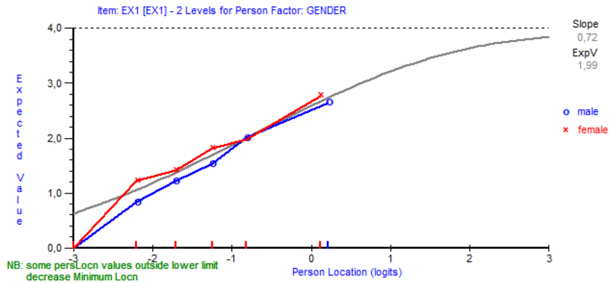
Fig 4. The item characteristic curve of item EX1 ( At work, I feel mentally exhausted ) for women and men in a sample from Check Republic (n=964).
