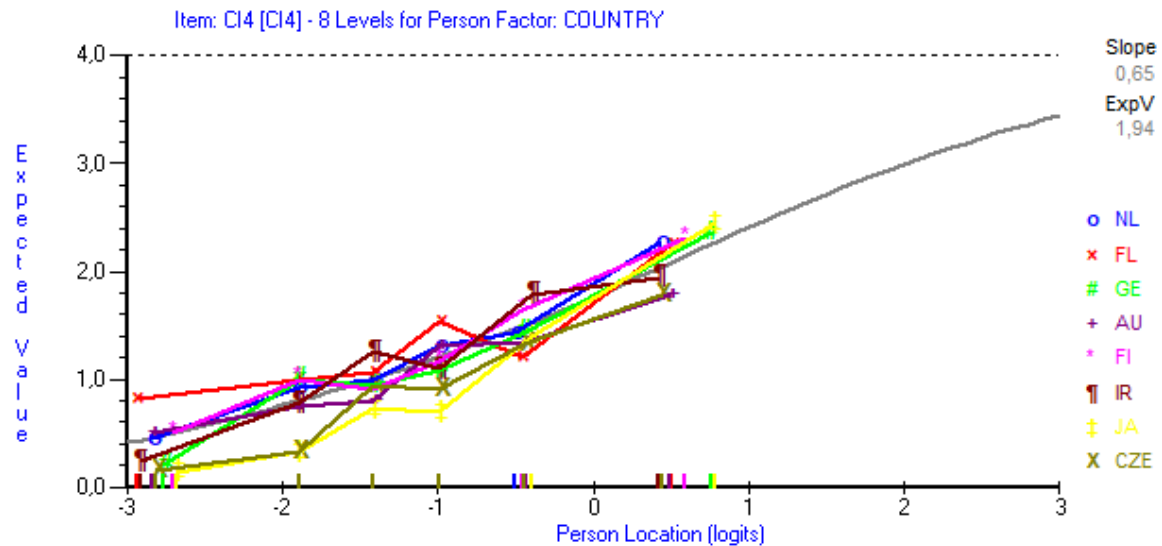
Fig 9. The item characteristic curve of item CI4 ( When I'm working, I have trouble concentrating ) for participants in different countries (NL= Netherlands, FL= Belgium, Flanders, GE=Germany, AU=Austria, FI=Finland, IR=Ireland, JA=Japan, CZE= Czech Republic) in a sample including 100 randomly selected participant from each country (n=800).
