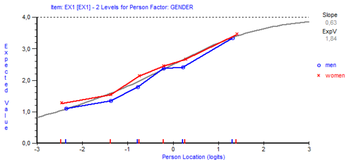
Fig 8. The item characteristic curve of item EX1 ( At work, I feel mentally exhausted ) for women and men in a sample from Japan (n=1028).
