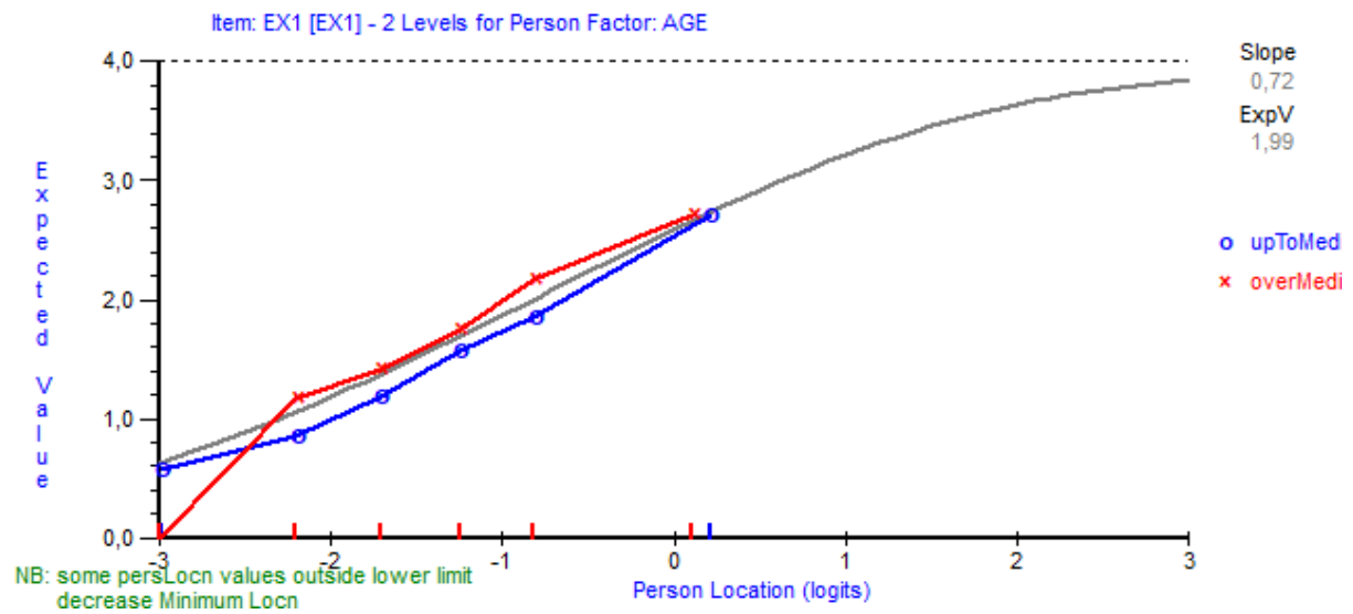
Fig 6. The item characteristic curve of item EX1 ( At work, I feel mentally exhausted ) for younger (up to median age of 42) and older (over median age of 42) participants in a sample from Check Republic (n=964).
