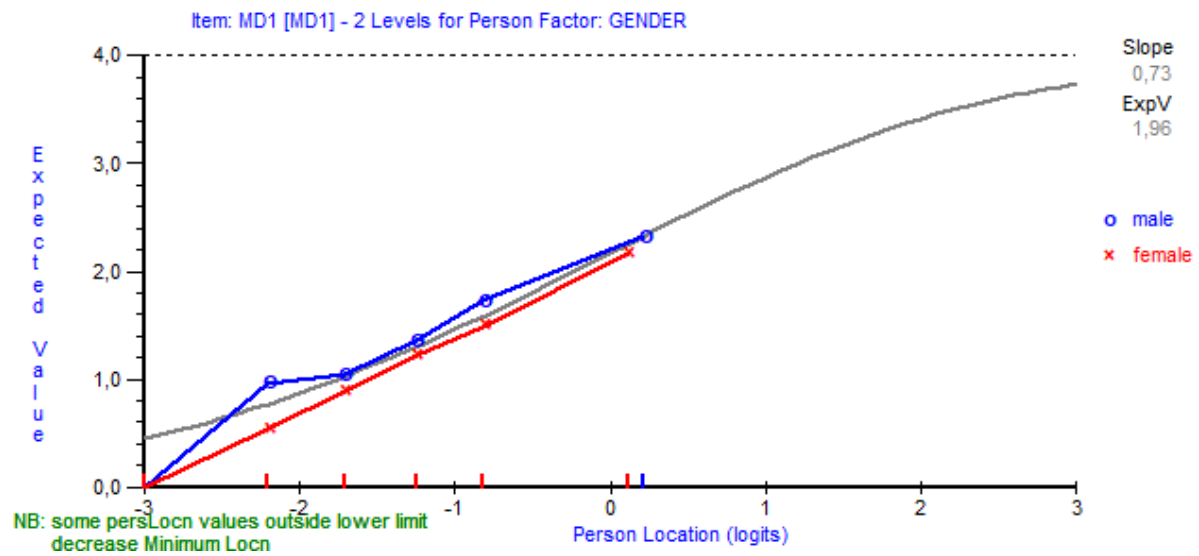
Fig 5. The item characteristic curve of item MD1 (I struggle to find any enthusiasm for my work) for women and men in a sample from Czech Republic (n=964).
