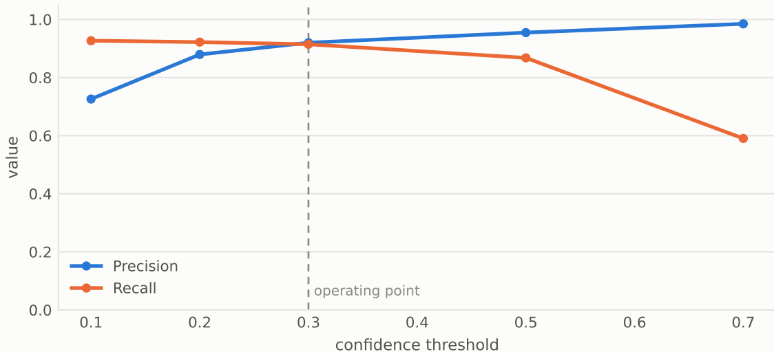
People in water: swimmer precision and recall against threshold
