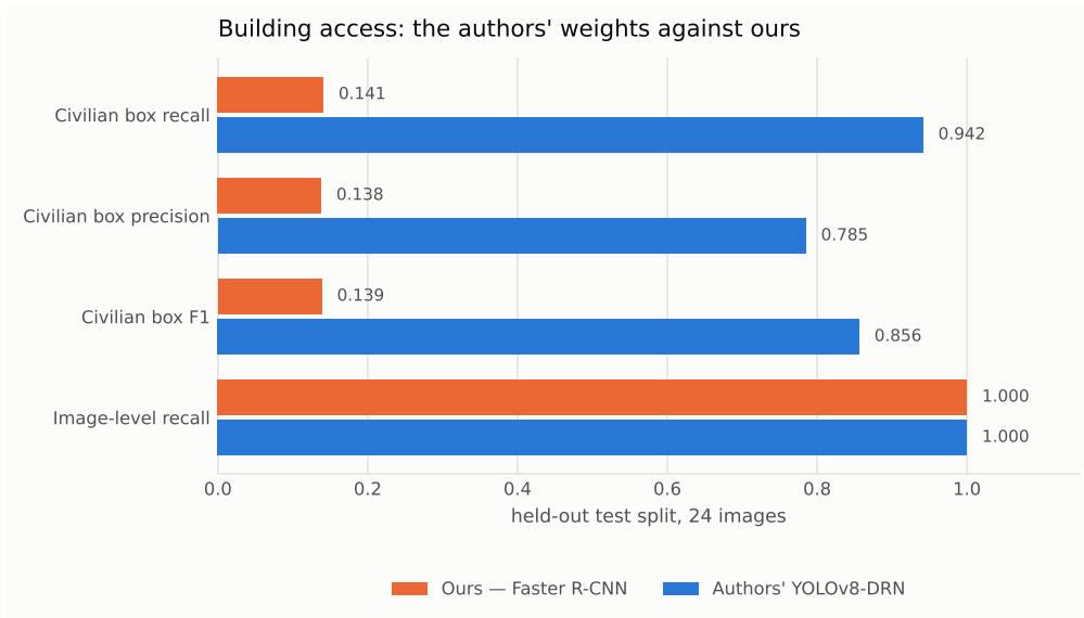
Figure 8. The two models on the identical held-out split with the identical metric. Image-level recall is 1.000 for both, which is exactly why image-level metrics alone are not enough (section 3.2.2): they hide a six-fold difference in whether the person was actually located.
