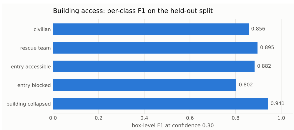
Figure 9. Per-class F_1 on the held-out split at confidence 0.30. Only civilian reaches the validator; the rest are operator context.
