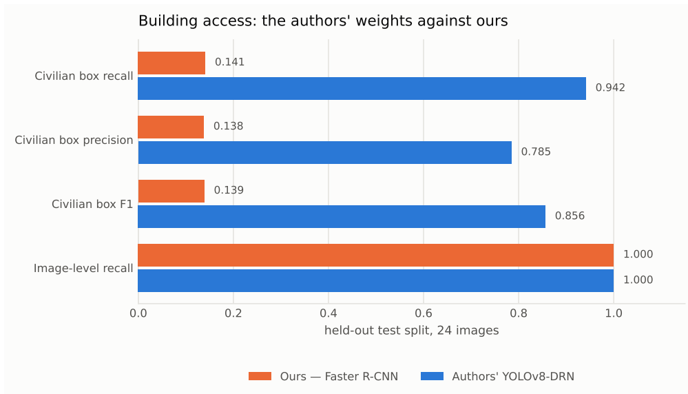
Figure 8. The two models on the identical held-out split with the identical metric. Image-level recall is 1.000 for both, which is exactly why image-level metrics alone are not enough (section 4.2): they hide a six-fold difference in whether the person was actually located.
