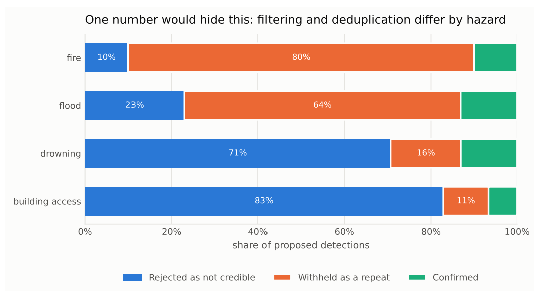
Figure 11. What the validator does with each hazard’s proposals. Fire’s headline suppression is almost entirely the system declining to re-announce one fire it had already found; building access’s is almost entirely filtering. Quoting a single figure would overstate the false-alarm contribution by a factor of eight on the fire clip.
