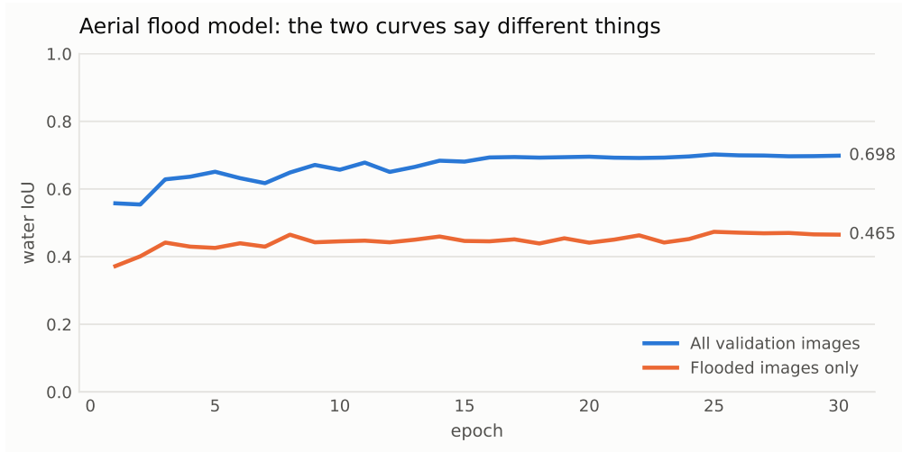
Figure 5. Training the aerial flood segmenter. The two curves are reported separately because only 51 of 398 labelled images are flooded; a single pooled IoU would be carried by dry scenes and would flatter the model on the one case it exists to handle.
