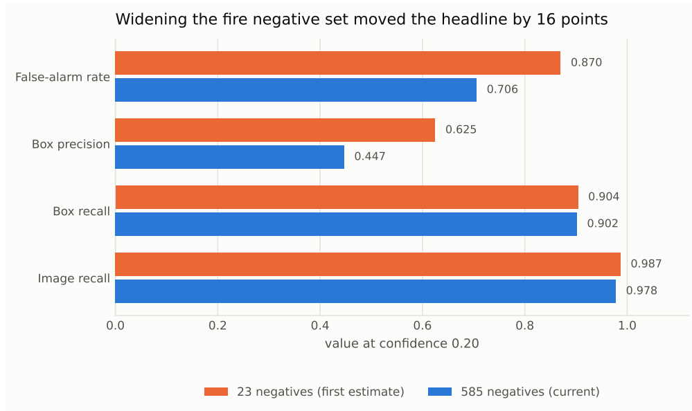
Figure 3. The same detector at the same threshold, measured against 23 negatives and then against 585. Recall barely moved; precision and the false-alarm rate both fell. This is what a small sample flattering a detector looks like.
