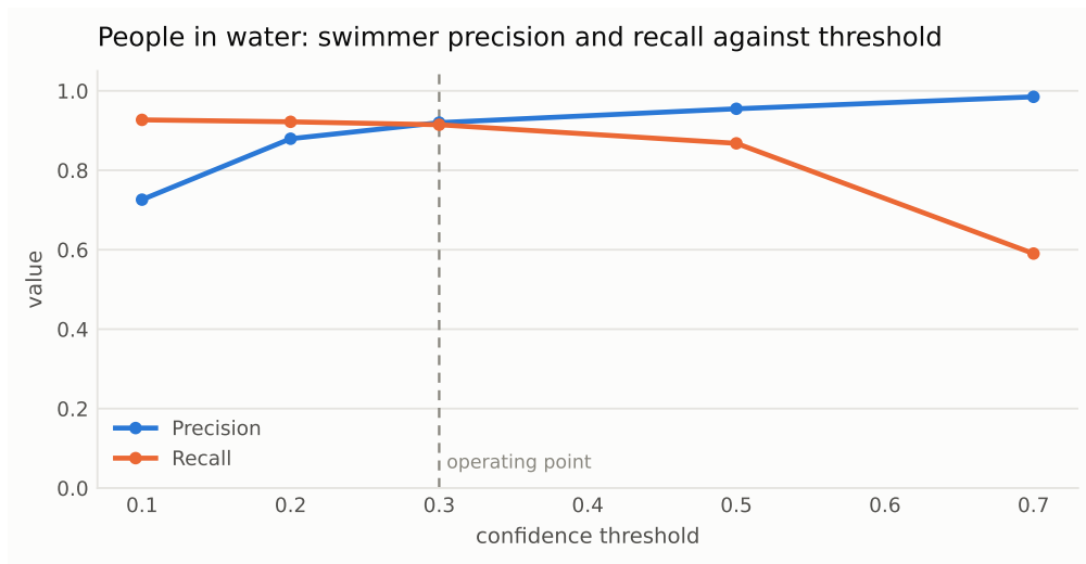
Figure 6. Swimmer precision and recall against the confidence threshold. The operating point is chosen where recall is still high, because the validator can discard a false alarm but nothing downstream can recover a person never detected — the same asymmetry that motivates \beta = 2 in eq. (6).
