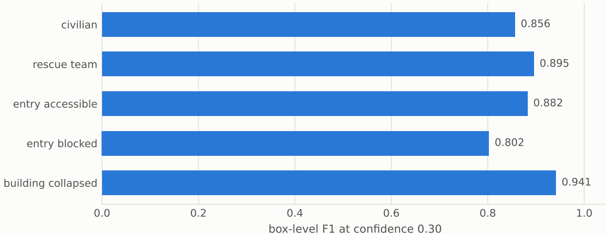
Building access: per-class F1 on the held-out split
