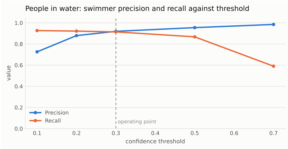
Figure 4. Swimmer precision and recall against the confidence threshold. The operating point is chosen where recall is still high, because the validator can discard a false alarm but nothing downstream can recover a person never detected — the same asymmetry that motivates \beta = 2 in eq. (6).
