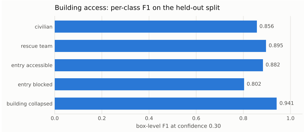
Figure 6. Per-class F_1 on the held-out split at confidence 0.30. Only civilian reaches the validator; the rest are operator context.
