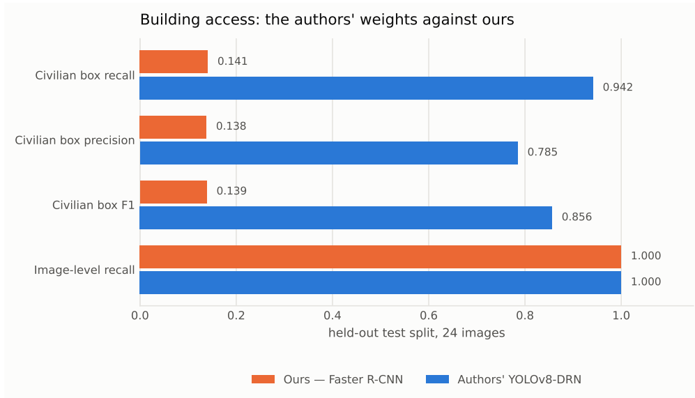
Figure 5. The two models on the identical held-out split with the identical metric. Image-level recall is 1.000 for both, which is exactly why image-level metrics alone are not enough (section 4.2): they hide a six-fold difference in whether the person was actually located.
