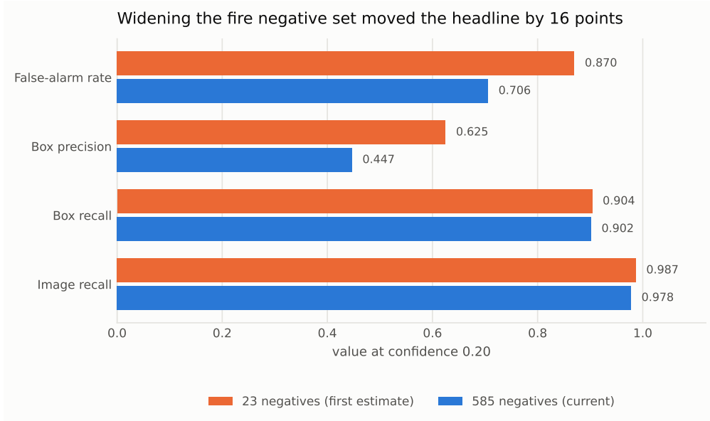
Figure 2. The same detector at the same threshold, measured against 23 negatives and then against 585. Recall barely moved; precision and the false-alarm rate both fell. This is what a small sample flattering a detector looks like.
