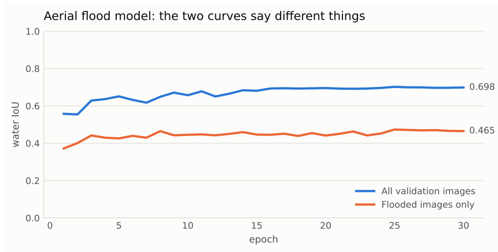
Figure 3. Training the aerial flood segmenter. The two curves are reported separately because only 51 of 398 labelled images are flooded; a single pooled IoU would be carried by dry scenes and would flatter the model on the one case it exists to handle.
