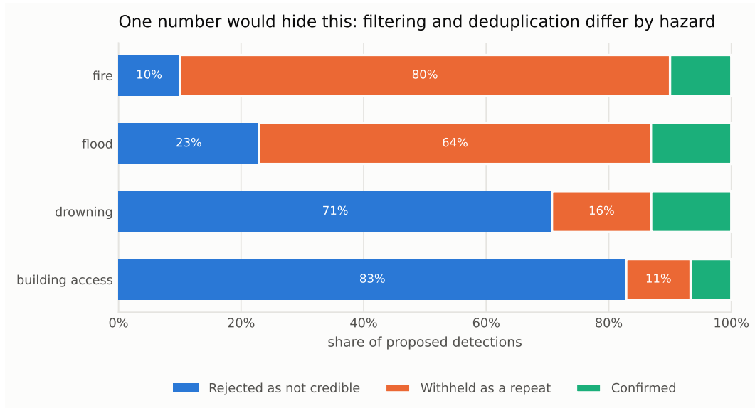
Figure 7. What the validator does with each hazard’s proposals. Fire’s headline suppression is almost entirely the system declining to re-announce one fire it had already found; building access’s is almost entirely filtering. Quoting a single figure would overstate the false-alarm contribution by a factor of eight on the fire clip.
