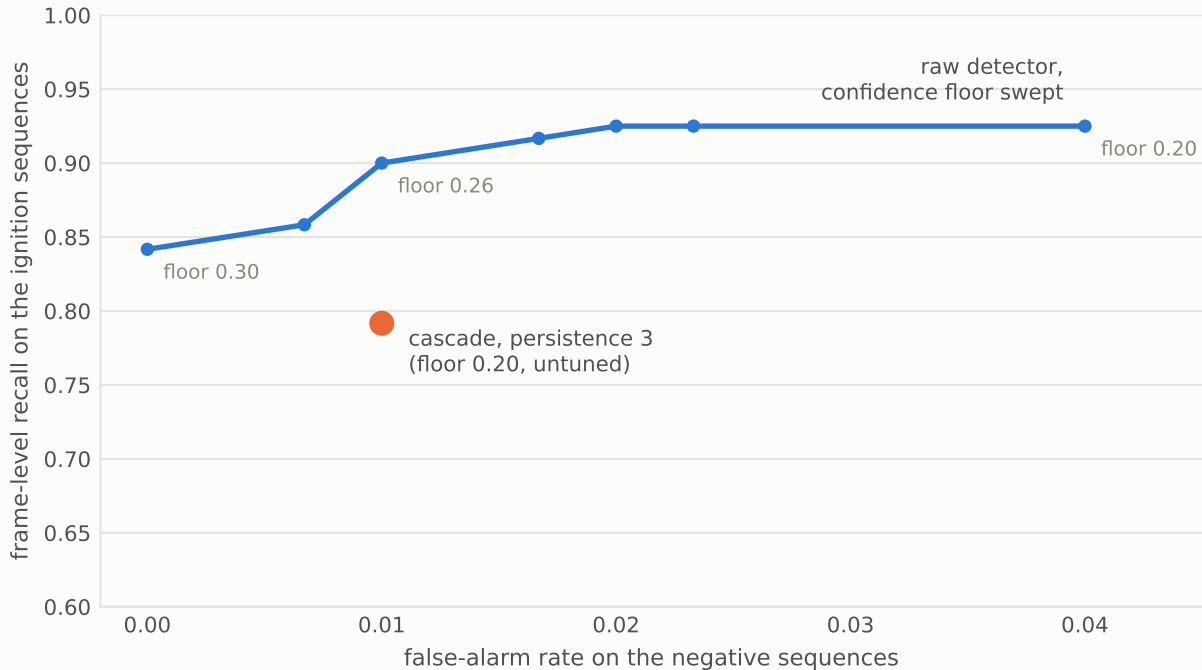
The obvious baseline, run: a tuned floor beats the cascade on this negative set
